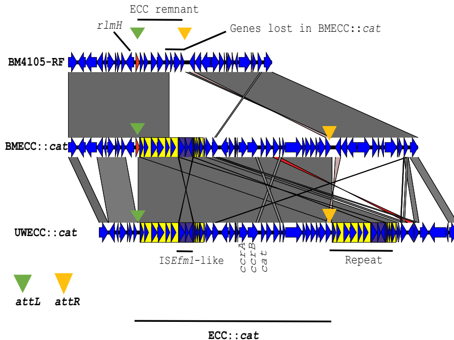
FIG 1 Pairwise alignment showing the genetic organization of chromosomal integration of ECC::cat . The insertion region in recipient BM4105-RF (top) is aligned with its transconjugant BMECC::cat (middle) after horizontal transfer from UWECC::cat (bottom). The ccrAB Ent genes and cat knock-in location are highlighted in UWECC::cat. Green and orange triangles show the locations of attL and attR sites, respectively. The rlmH gene is drawn in red. Ten-kilobase direct repeats in UWECC::cat are highlighted in yellow, and the ISEffm1 element is highlighted in purple.
