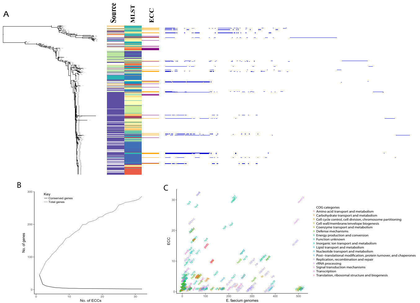
FIG 3 Presence of ECC in enterococcal genomes, pan-genome analyses of genes present in ECC. (A) Phandango-generated overview of WGS tree of 516 E. faecium genomes created by pansnp, with annotated MLST profiles as shown by colors. The presence of ECC elements (yellow for full elements and purple for ccrAB Ent -positive, fragmented assembly) and source of isolation (violet for human, turquoise for lab strain, green for animal, yellow for environment, orange for food) are shown by different colors. To the right, pan-genome plot in blue showing genes in ECCs, sorted vertically by the position of ECC-positive strain in phylogeny and horizontally by gene prevalence with the most abundant genes to the left. (B) Graph showing accumulating number of accessory genes and conserved genes in ECCs. (C) Scatter plot of genes annotated by eggNOG, plotted in coordinates corresponding to occurrences of gene in ECCs (y axis) and E. faecium genomes (x axis), with colors corresponding to the assigned cluster of orthologous group (COG).
