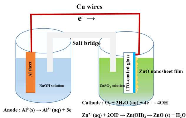
Fig. 1 The schematic drawing of the experimental setup used for the fabrication of hexagonal ZnO nanosheet films
