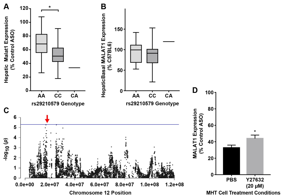
Fig 7. Identification and validation of Rock2 in ASO activity. (A) Distribution of hepatic Malat1 expression based on genotype distribution at rs29210579. Box and whisker plot depicting mean and distribution, unpaired t-test, * p \leq 0.05 (B) Distribution of basal hepatic Malat1 expression based on genotype distribution at rs29210579. Box and whisker plot depicting mean and distribution. (C) Chromosome 12 plot for Rock2 displaying all significant SNPs ( -\log_{10}(p) ) for ASO efficacy. Red arrow indicates position of gene. (D) MHT cells were incubated with Malat1 ASO and control ASO in presence and absence of 20 \mu\text{M} Y27632. After 24 hrs, Malat1 ASO potency was assessed in all samples. MHT cells exhibit lower reduction in Malat1 expression with Y27632 as compared to PBS. Data shows mean \pm S.E.M (% control ASO) with two-way ANOVA and Bonferroni's multiple comparison test. * p \leq 0.05 .
