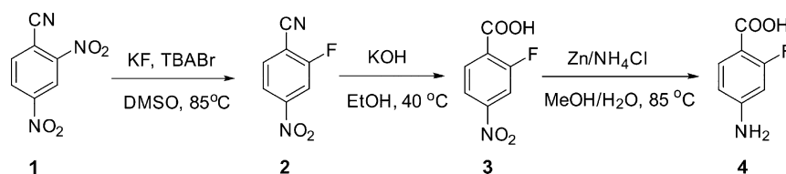
Scheme 2. Synthesis of 2-F-PABA from 2,4-Dinitrobenzonitrile
