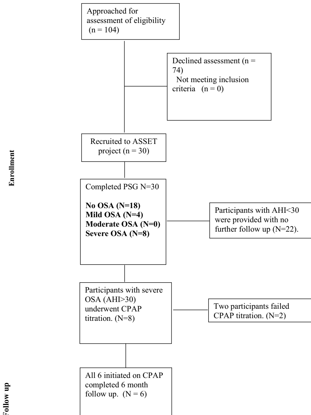
Fig. 1. Consort diagram.
