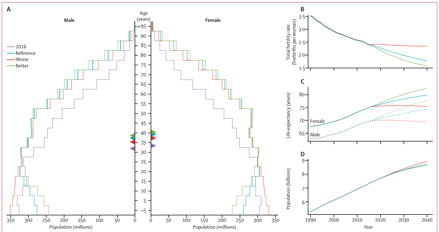
Figure 3: Global distribution of population in 2016 and 2040 reference forecasts, 2040 better health scenario, and 2040 worse health scenario
