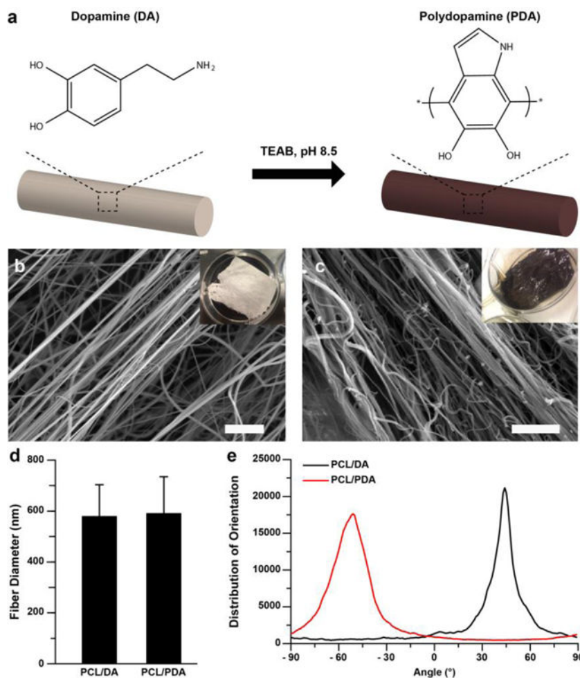
Figure 1. Nanofiber fabrication. (a) Schematic illustration of polymerization of PCL/DA into PCL/PDA through treatment with triethylammonium bicarbonate (TEAB, pH 8.5) buffer. (b–c) SEM images of b) PCL/DA and c) PCL/PDA. Insets indicate macroscopic images of nanofibers. Scales are 10 \mu\text{m} . d) Fiber diameter analysis. n=4 . e) Fiber directionality calculated from (b–c) SEM images.
