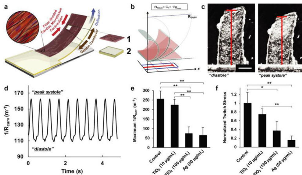
Figure 4. Measuring contractile stress using fiber-coated gelatin MPS. a) Principle sketch of a fiber-coated MPS with cardiomyocytes. Constituent layer 1: engineered cardiac tissue within nanofiber scaffolds and 2: gelatin thin film; see Electronic Supplementary Material Movie 2 for a representative video of a fiber-coated gelatin MPS seeded with contracting NRVMs. b) Schematic diagram showing the extrapolation of x-projections of cantilever deflection in 2D and its correlation to R_{\text{curv}} . c) Optical images showing the cantilever motions associated to cardiomyocyte diastole and systole. Scale is 1 mm. d) Representative plot of the geometric readout from the optical recording of MPS motion over time, under 2 Hz pacing. e–f) Comparison of (e) maximum 1/R_{\text{curv}} and (f) normalized twitch stress values calculated from Day 5 cardiac MPS samples under different ENM exposure conditions (48 h after ENM addition, 2 Hz pacing at 10 V). For statistical comparison, * p < 0.10 and ** p < 0.05 , n = 10 for control, n = 6 for 10 and 100 \mu\text{g}/\text{mL} and \text{TiO}_2 , and n = 7 for Ag (50 \mu\text{g}/\text{mL} ).
