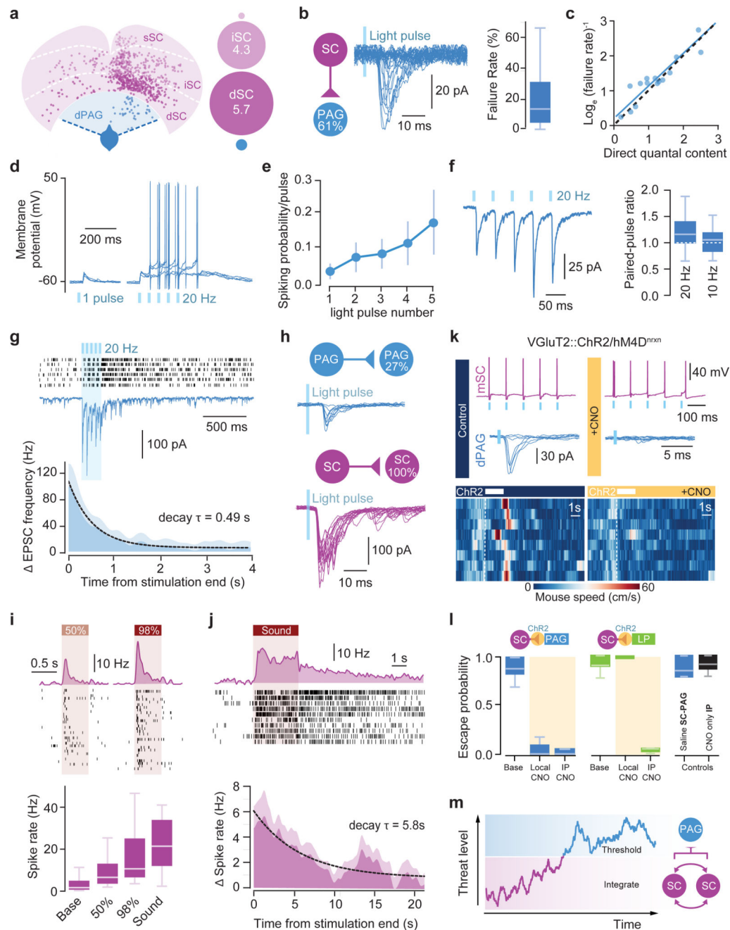
Figure 4. Neural circuit and biophysical mechanisms for computing escape behaviour a , Left, dPAG VGlut2 + (blue) and presynaptic cells (pink) from rabies tracing, for deep (dSC), intermediate (iSC) and superficial SC (sSC). Right, SC:dPAG convergence ratios for single dPAG cells. b , mSC-dPAG connectivity (left; n=79, N=21), example traces (middle), and failures summary (right, n=8, N=7). c , Direct quantal content versus estimation from failure rate (fit slope = 0.92, 95% CI [0.74, 1.1]; n=15). Blue line: linear fit, dashes: unity line (see Methods). d , dPAG voltage response to dSC stimulation. e , Spiking probability summary (n=20 N=10, plot shows mean and SEM). f , Example average trace (left) and
