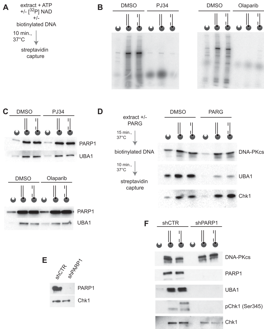
Figure 3. pADPr chains are required for UBA1 recruitment. (A) Reaction mixtures were incubated with [ 32 P]-labelled NAD, and DNA-bound proteins were pulled down and resolved by PAGE. Poly(ADP-ribosyl)ated proteins were revealed by autoradiography. (B) Autoradiography of proteins poly(ADP-ribosyl)ated in nuclear extracts and isolated with the indicated DNA substrates represented schematically. Biotin (black circles) and streptavidin-coated beads (dented grey circles) are shown. When indicated, reactions were performed in the presence of the PARP1 inhibitors PJ34 or olaparib. (C) Western blot analysis of the indicated proteins isolated with biotinylated DNA substrates from reaction mixtures supplemented, when indicated, with PJ34 or olaparib. (D) Nuclear extracts were pretreated with PARG when indicated and incubated with DNA substrates. The indicated proteins were isolated by DNA pull-down and revealed by Western blotting. (E) Western blot analysis of PARP1 and Chk1 in nuclear extracts prepared from cells treated with anti-luciferase (shCTR) or anti-PARP1 (shPARP1) shRNAs. (F) The indicated proteins were isolated along with biotinylated DNA substrates after incubation in protein extracts from cells treated with control (shCTR) or anti-PARP1 shRNAs, as indicated.
