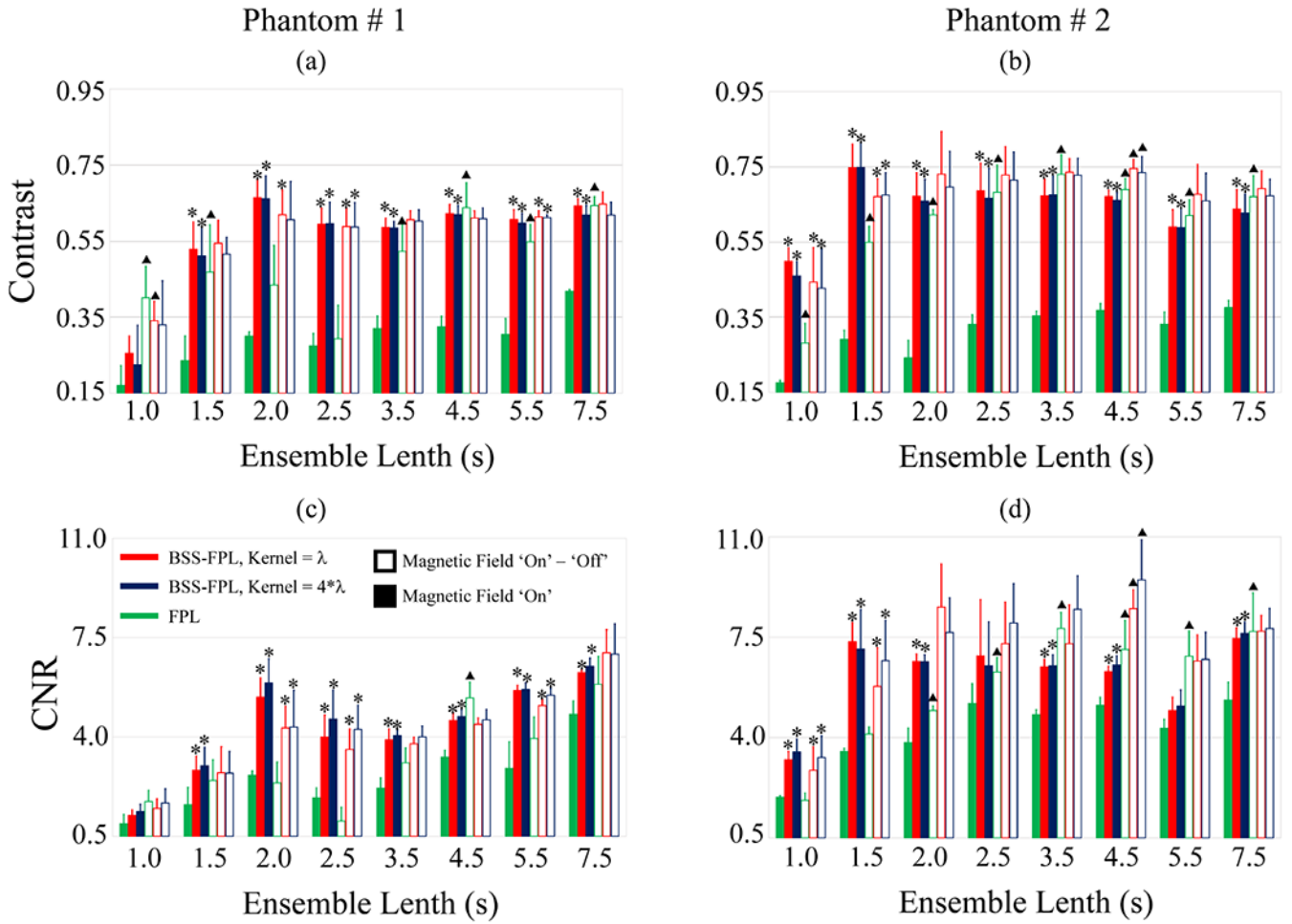
Fig. 6. Contrast (top row) and CNR (bottom row) of inclusions in phantoms #1 (a, c) and #2 (b, d) as a function of ensemble lengths. Data are plotted as median + 0.5 × interquartile range over 5 acquisitions in different elevational planes in each phantom. Green, red, and blue represent FPL, BSS-FPL with kernel length = \lambda , and 4\lambda , respectively. Filled and open bars represent magnetic field ‘on’ (B-on) and magnetic field ‘on’ – ‘off’ (background subtracted) data, respectively. Asterisks (*) represents significantly different ( p < 0.05 ) values between FPL versus BSS-FPL with kernel length = \lambda and 4\lambda . Triangles (▲) represent significantly different ( p < 0.05 ) values between magnetic field B-on versus background subtracted data.
