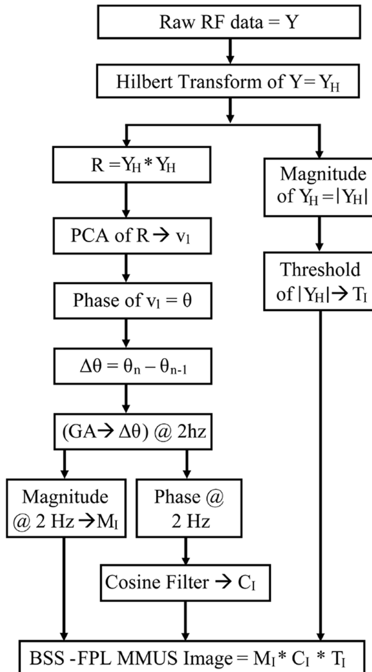
Fig. 1. Steps for detecting motion in MMUS imaging using the BSS-FPL algorithm. PCA = principal component analysis; v_1 = the most energetic Eigen vectors; n = 2, 3, \dots , ensemble length, GA = Goertzel algorithm.
