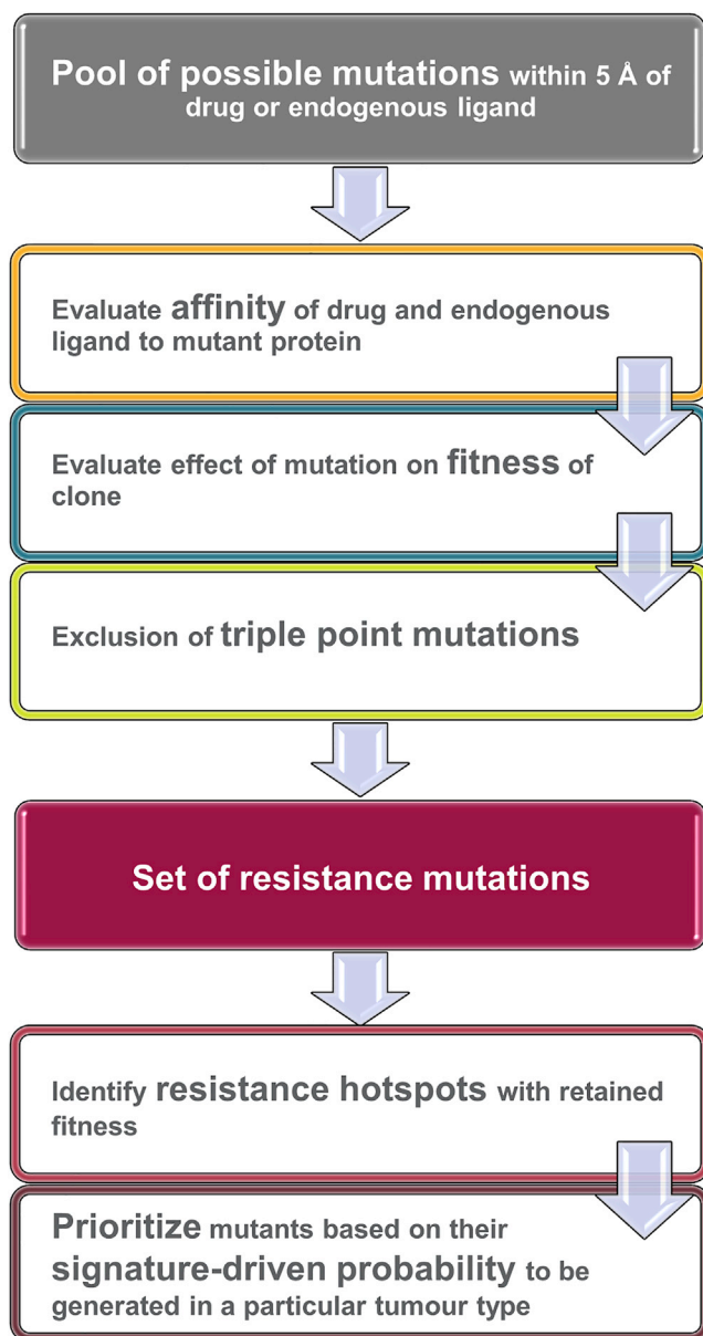
Figure 1. Workflow
