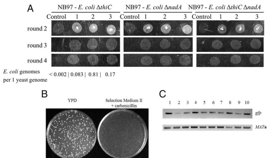
Fig. 3. S. cerevisiae – E. coli chimeras have a partially rescued respiration-competent phenotype. (A) Growth of S. cerevisiae cox2-60 – E. coli chimeras on medium containing glycerol as the sole carbon source, selection medium III. No growth was observed for parent cox2-60 yeast lacking intracellular E. coli (control). Three different chimera colonies growing during successive rounds of plating are shown for each S. cerevisiae – E. coli chimera. Number of E. coli genomes per one yeast genome was determined by qPCR for E. coli \Delta thiC chimeras from the fourth round of growth. (B) A single cell suspension of S. cerevisiae cox2-60 – E. coli \Delta nadA chimera culture formed a comparable number of colonies on non-selective (YPD) and selective medium (selection medium II) plates. (C) Total DNAs isolated from colonies grown on selection medium II in B contain E. coli -encoded gfp gene. Ten random colonies (labeled 1–10) were PCR amplified for presence of gfp and MATa genes.
