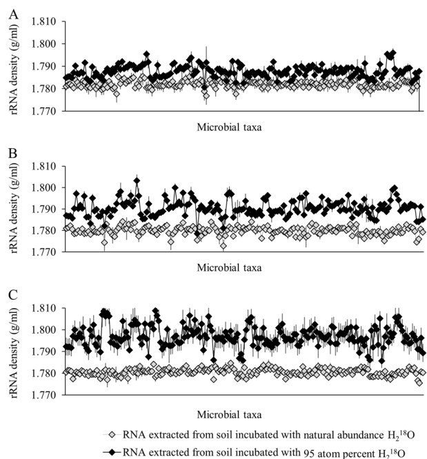
Fig. 1 Densities of rRNA extracted from soil incubated with 95 atom % \text{H}_2^{18}\text{O} ( \blacklozenge ) or natural abundance \text{H}_2^{18}\text{O} ( \blacklozenge ) on three time points. a rRNA densities of taxa detected on day 1, b , c rRNA densities of taxa detected on day 4 and 8, respectively. Taxa are ranked by the same alphabetical order in each panel. Symbols represent means \pm standard deviations
