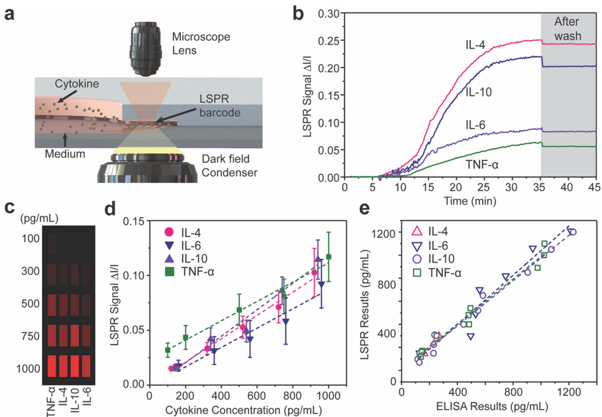
Figure 2. Label-free and multiplex nanoplasmonic measurement of cell-secreted cytokines.
