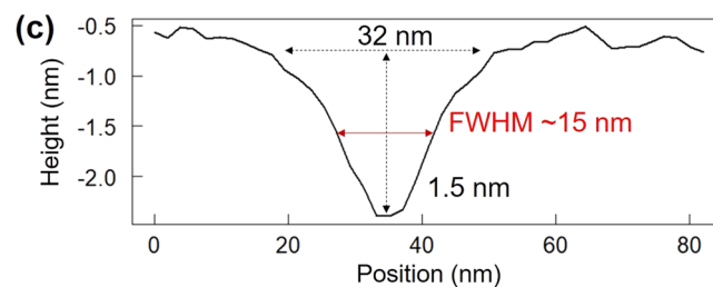
Figure 1. Local photoisomerization in a slightly coloured photochromic crystal. (c) Line profile obtained along the white line in (b).
