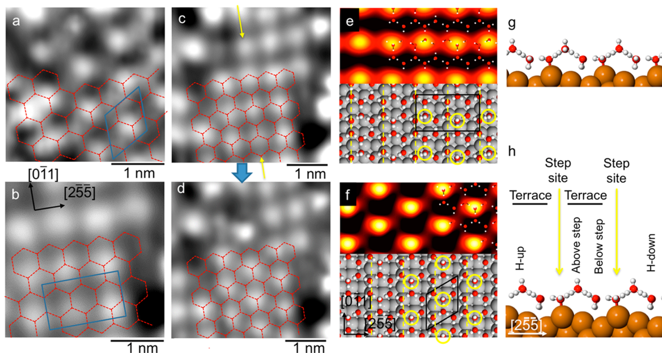
Figure 3. STM images for the 1 ML water structure formed at 138 K showing the formation of a hexagonal network containing water adsorbed with some OH groups pointing away from the surface. (a) Detail of a region with a hexagonal arrangement of bright features in a (3\ 0, -1\ 1) repeat and (b) a region with bright features aligned along [2\bar{5}5] in a doubled, rectangular (3\ 0, 1\ 2) repeat that crosses two steps. (c and d) Images of the same region showing a structural change from the rectangular arrangement (c) to hexagonal (d), achieved during scanning by increasing the tunneling current to bring the tip close to the surface. The sites marked by the yellow arrows move up one Cu unit leaving the remaining water network unperturbed, as indicated by the dashed hexagonal network. (e,g and f,h) STM simulations (0.1 V) and DFT structures for arrangements containing one H-up water per unit cell (see SI, structures S4Y and S3D) either in or out of phase on adjacent Cu terraces, with adsorption energies of -75.1 and -75.2 kJ/mol, respectively. The position of the H-up water molecules is indicated by the yellow circles. STM scan direction is vertical with (a) 0.11 V, 41 pA; (b,c) 0.11 V, 21 pA; (d) 53 mV, 21 pA.
