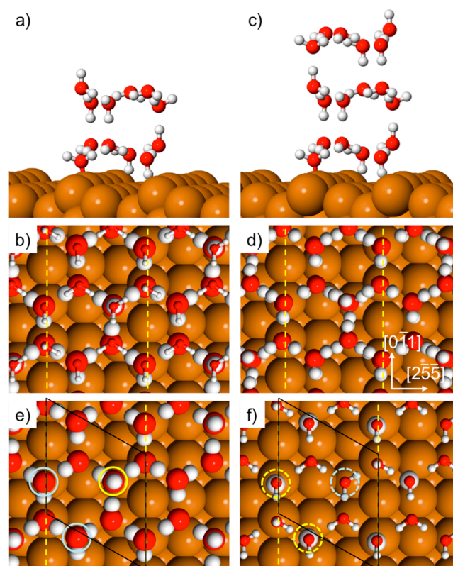
Figure 5. Calculated structures showing the best 2 and 3 layer structures found in a (3\ 0, -1\ 1) unit cell. Side and top view of (a–b) 2 ML water and (c–d) 3 ML water (adsorption energy -71.8 and -71.6\ \text{kJ/mol} respectively). The top frames show a single unit cell of water, while the top layer in (b) is reduced in size. Frames (e,f) show the first and second layers of the 2 layer structure separately. The three first layer sites (e) that link the two layers are circled with the H-up donor in yellow and the acceptor sites in blue. Frame (f) shows the corresponding second layer donor/acceptor sites highlighted by dashed circles, with the H donors enlarged. Copper step sites are indicated by the yellow dashed lines.
