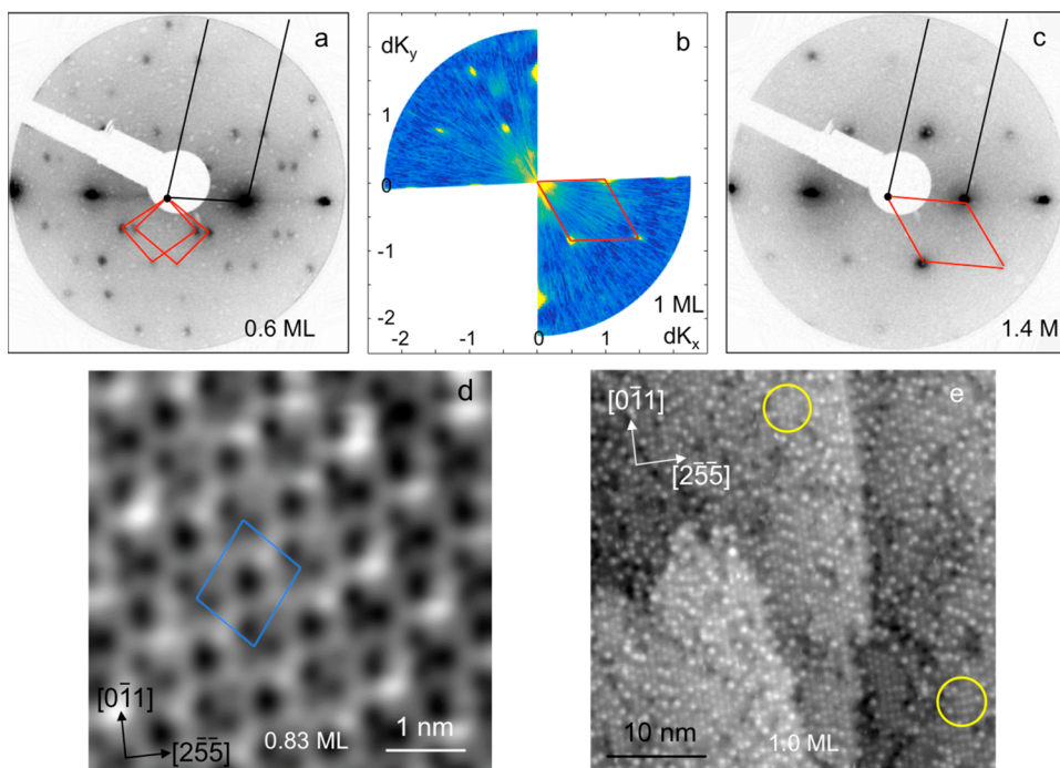
Figure 2. Diffraction patterns and STM images showing the change in structure as the first layer saturates with water. (a) LEED pattern (40 eV, 10 nA) showing formation of the (3\ 1, -3\ 1) structure for water coverage \leq 0.83 ML, (b) HAS (recorded at an energy of 9.69 meV), and (c) LEED (40 eV, 10 nA) showing the formation of an ordered (3\ 0, -1\ 1) water film at \geq 1 ML water. The Cu(511) reciprocal unit cell is shown by the black lines, while the red lines show that for water. (d) STM image of the (3\ 1, -3\ 1) structure ( -0.11 V, 100 pA) and (e) the (3\ 0, -1\ 1) structure (0.11 V and 21 pA). The yellow circles show regions where the bright features are arranged locally into a hexagonal pattern (top) or a rectangular arrangement (bottom). The water coverage is marked on the images, which are all recorded at 77 K after annealing the surface to 138 K, except (b) which is recorded at 120 K (see Methods for further details).
