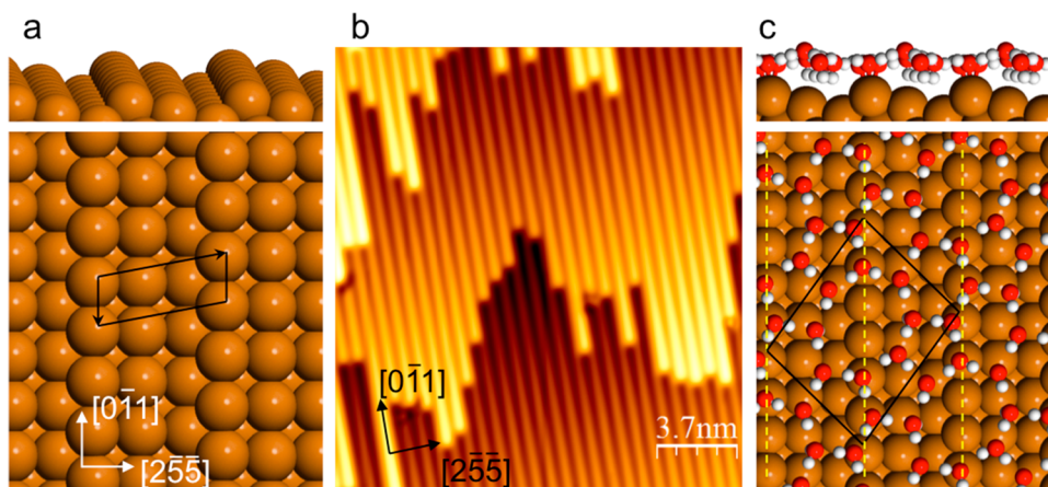
Figure 1. Structural model for the bare Cu(511) surface and the low coverage water phase. (a) Model showing the close packed Cu steps separated by (100) terraces and (b) an STM image showing the regular array of steps aligned along the [0\bar{1}1] direction. (c) Structural model for the water monolayer formed at low coverage, 28 showing the (31, -31) unit cell and Cu steps indicated by the dashed lines.
