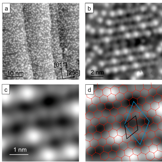
Figure 4. STM images showing second layer water forming a continuous 2D layer across the entire surface. (a) Large scale STM image of \sim 2 ML water after annealing at 135 K. (b) Detail showing the bright features preferentially aligning orthogonal to the steps. (c) Portion of the surface with fewer bright features where the second layer water network is visible. (d) Original (3\ 0, -1\ 1) first layer network superimposed (red hexagons shown with black unit cell), along with the (5\ 1, -4\ 1) unit cell (blue) that represents the commensurate second layer superstructure. (a) 0.1 V, 21 pA; (b–d) 0.1 V, 41 pA.
