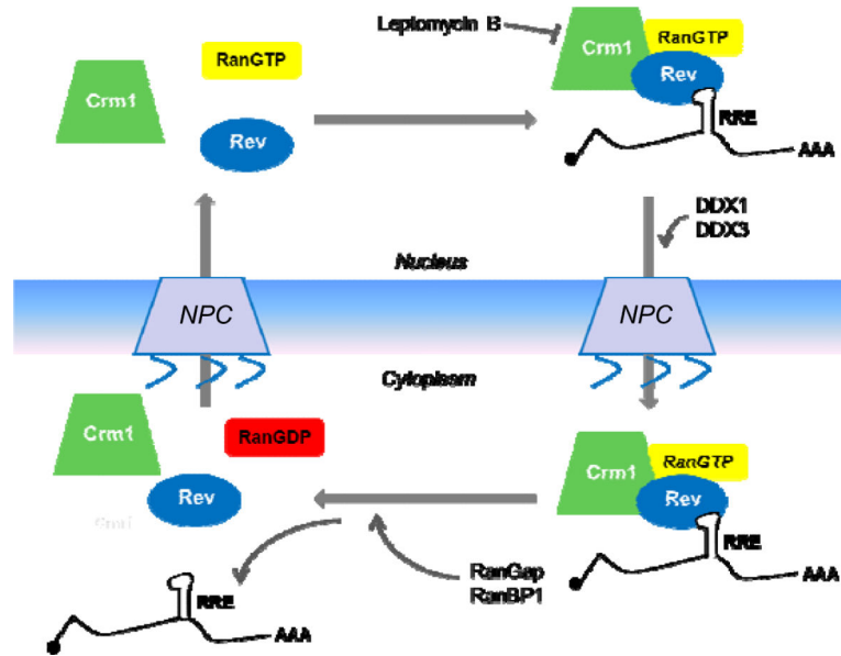
Figure 2. Nuclear export mechanism of full-length and partially spliced HIV-1 RNA Viral protein Rev serves as a bridge that recruits Crm1 and RanGTP to intron-containing HIV-1 RNAs by binding to the RRE. The Rev-RRE-Crm1-RanGTP complex moves through the nuclear pore complex (NPC). Once in cytoplasm, RanGap and RanBP1 lead to hydrolysis of Ran-associated GTP into GDP causing the dissociation of the export complex and the release of HIV-1 RNA. Although not shown, other host proteins, such as DDX3, may be involved in the nuclear export process (Figure not drawn to scale).
