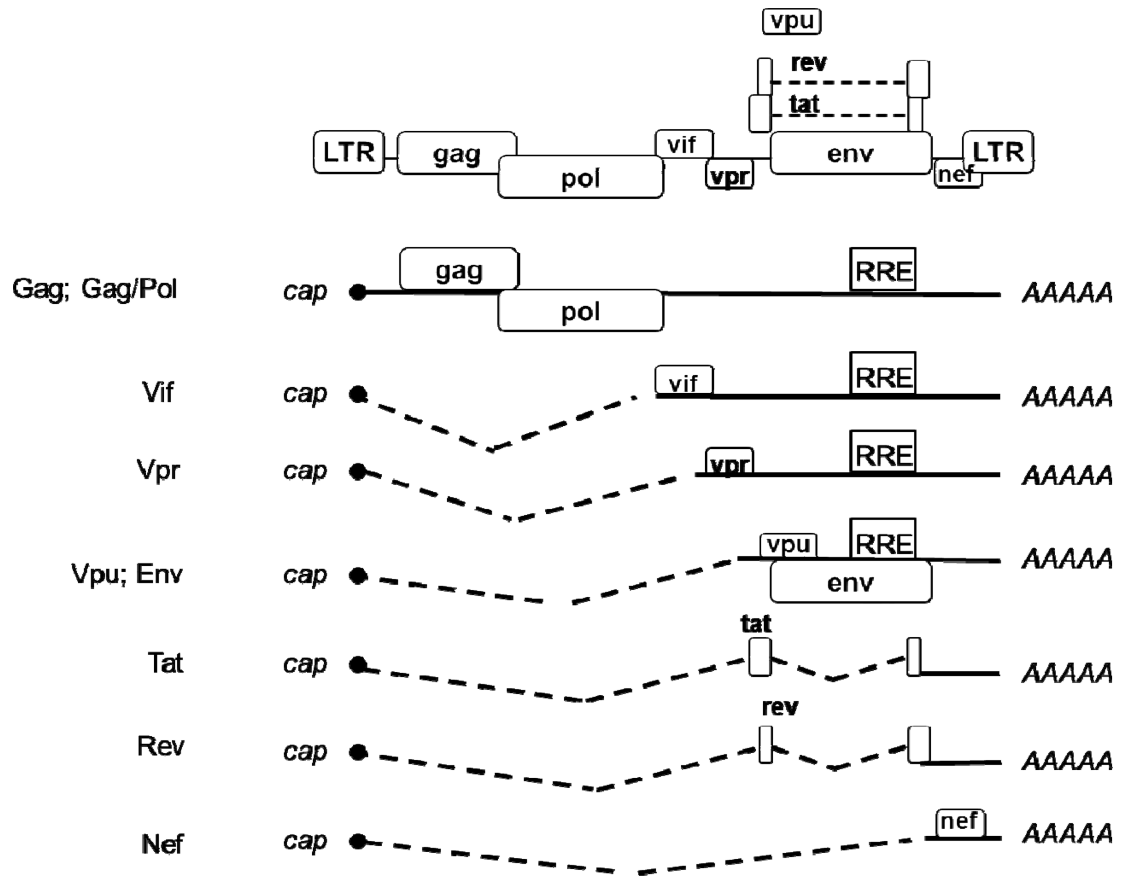
Figure 1. HIV-1 generates multiple RNA species through splicing
