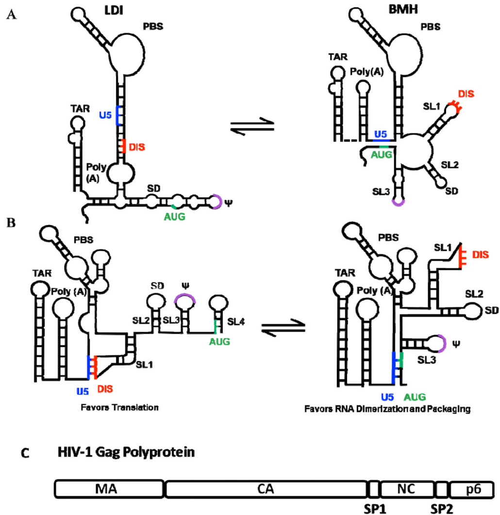
Figure 3. Cis- and trans- factors of HIV-1 RNA packaging
