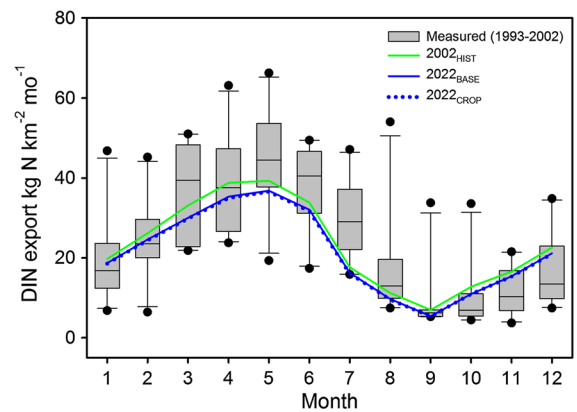
Fig. 4 Upper panel comparison of measured ( gray bars ) and model-derived ( lines ) dissolved inorganic nitrogen (DIN) export ( \text{kg N km}^{-2} \text{mo}^{-1} ) for the Mississippi River Basin. Box plot shows median value ( horizontal lines ), 25th and 75th percentile ( box outline ), 10th and 90th percentile ( error bars ), and 5th and 95th percentile ( solid points )
