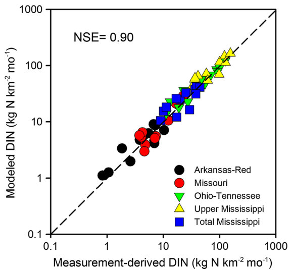
Fig. 3 Comparison of measured and model-derived dissolved inorganic nitrogen (DIN) yields ( \text{kg N km}^{-2} \text{mo}^{-1} ) for the Mississippi River Basin and four major sub-basins. NSE is Nash–Sutcliffe efficiency. The diagonal line indicates 1:1
