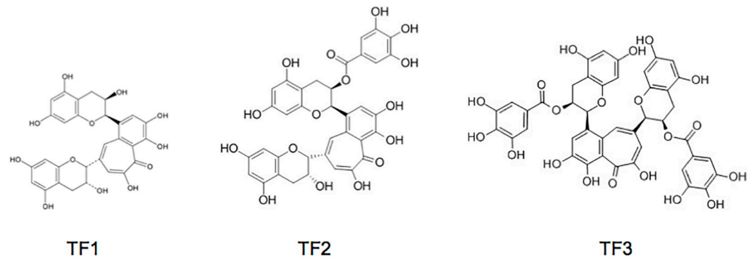
Fig 1. Chemical structures of theaflavins extracted from black tea.
