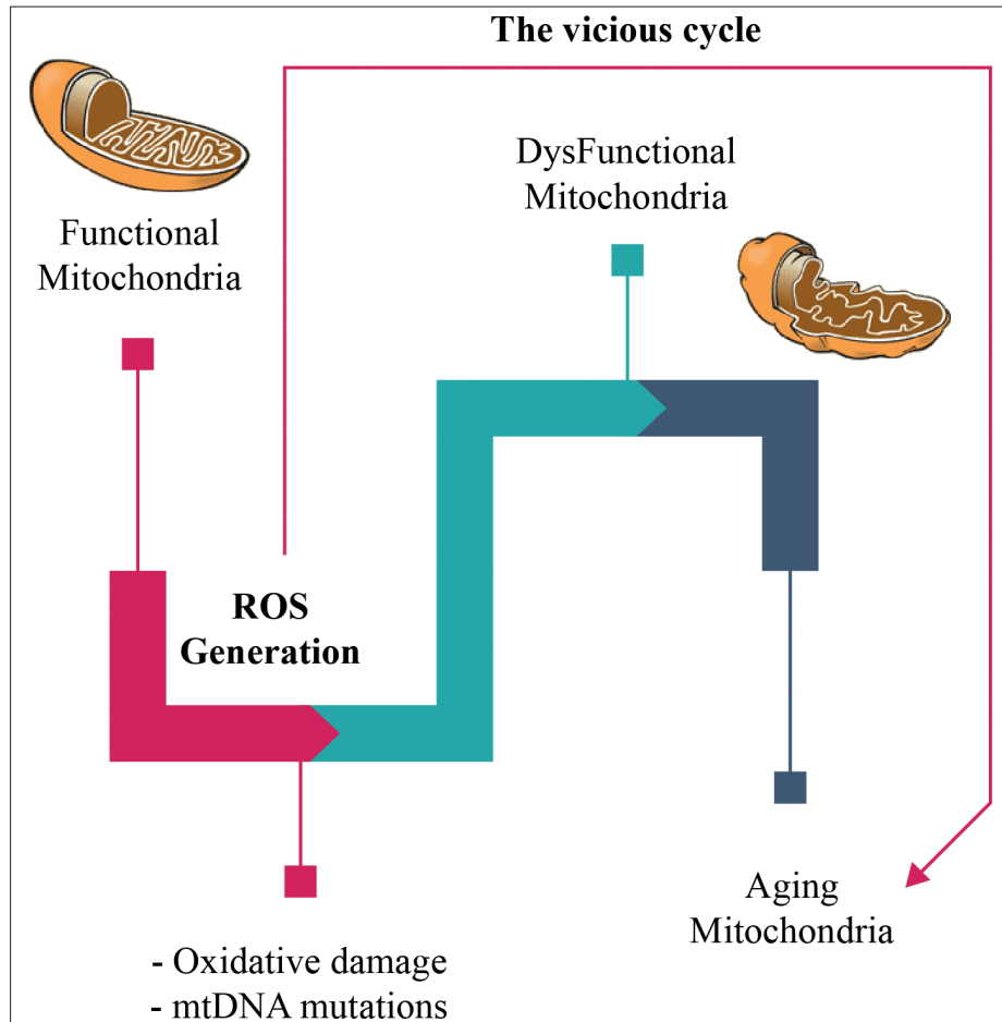
Figure 2. Schematic representation of the mitochondrial free radical theory
