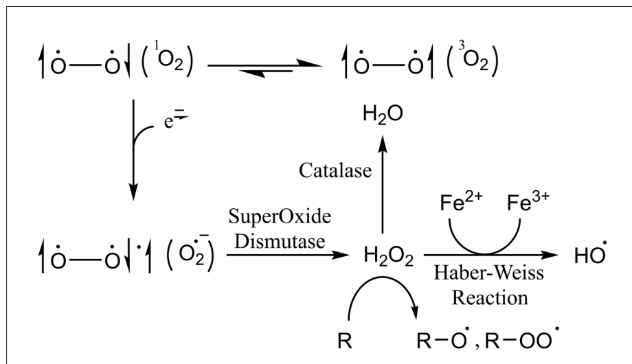
Figure 1. Chemistry of in vivo conversion of oxygen molecule to several ROS
