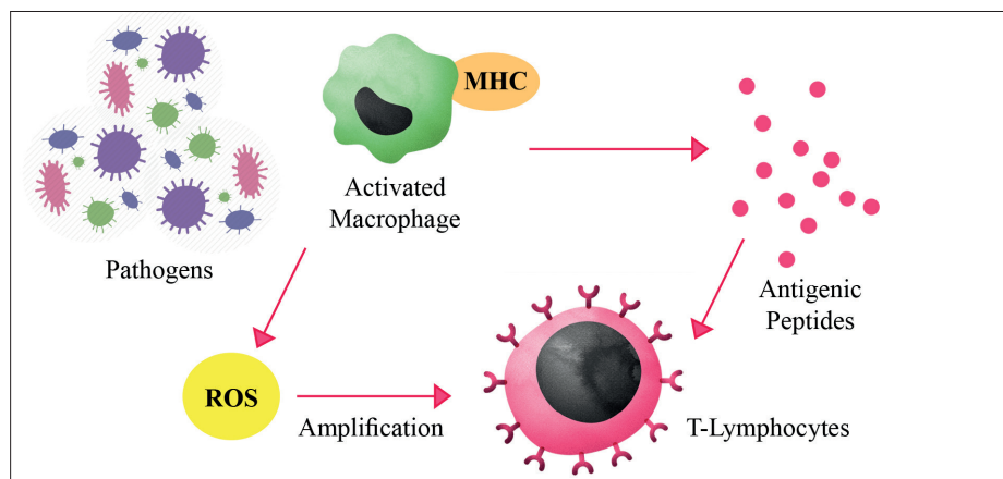
Figure 3. Functions of ROS in immunological response against environmental pathogens. Mass production of ROS by activated macrophages provides a first line of defense against environmental pathogens
