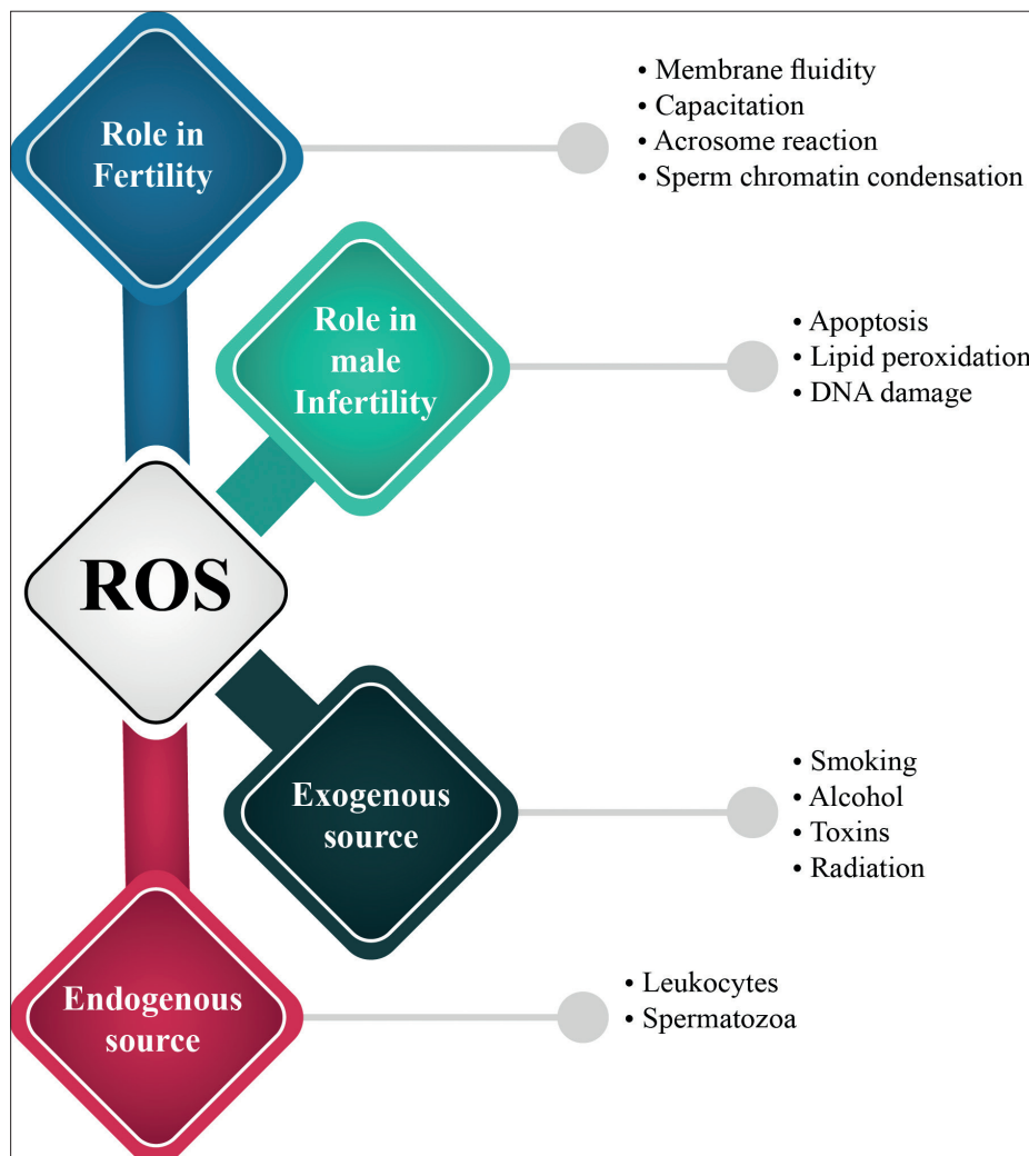
Figure 4. Roles of ROS in fertility and infertility
