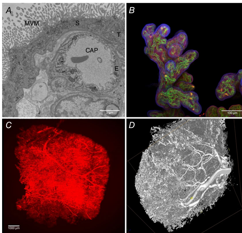
Figure 3. Evaluating imaging techniques for use in assessing placental structure
