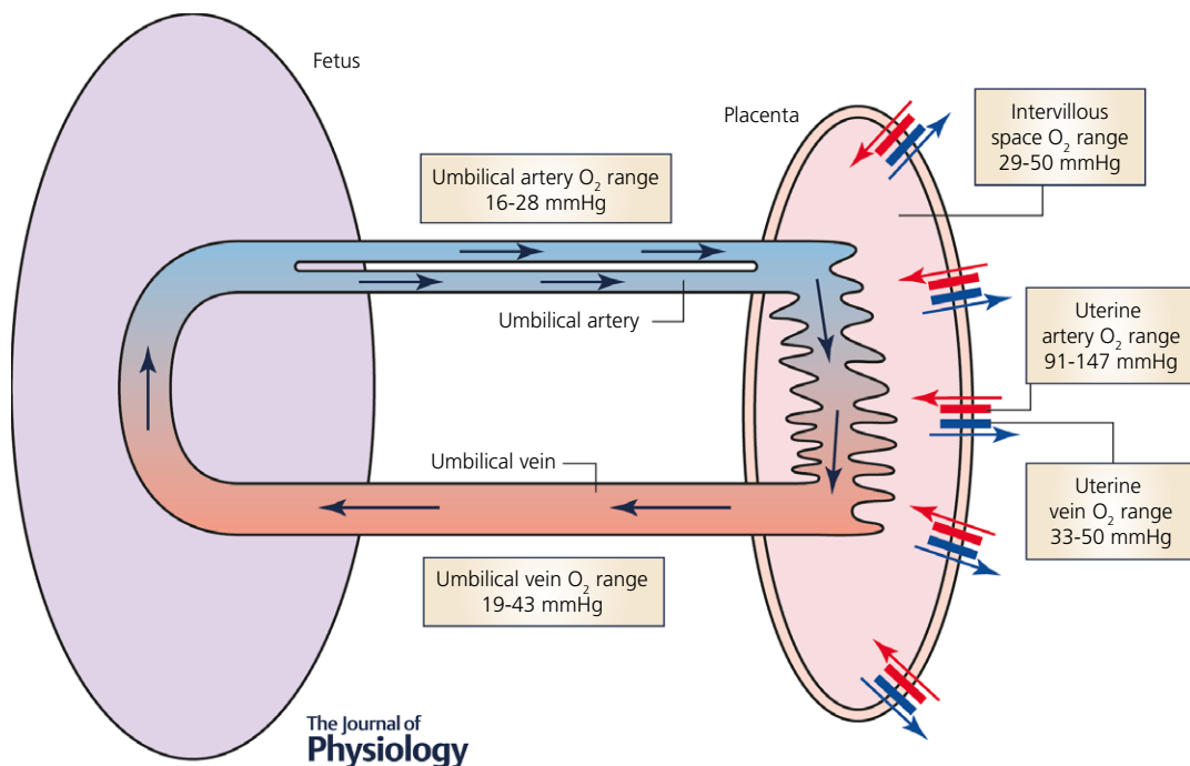
Figure 1. Simplified schematic diagram of the maternal and fetal placental circulations, showing the major compartments and published attributed in vivo oxygen values (see Table 1)
