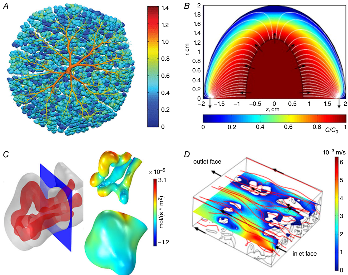
Figure 4. Mathematical modelling of human placental perfusion and oxygenation at different scales A, variability of perfusion in a fetoplacental vascular network (colour scale shows pressure for chorionic vessels and relative capillary flow for terminal capillaries, plotted as spheres) (Clark et al. 2015). B, distribution of a passive solute in the intervillous space of a single placental lobule (Chernyavsky et al. 2010). C, oxygen flux distribution over the capillary and syncytiotrophoblast surfaces of a single terminal villus (Pearce et al. 2016). D, microscopic flow in the intervillous space (Perazzolo et al. 2017). Images are reproduced with permission, subject to the respective copyrights.
