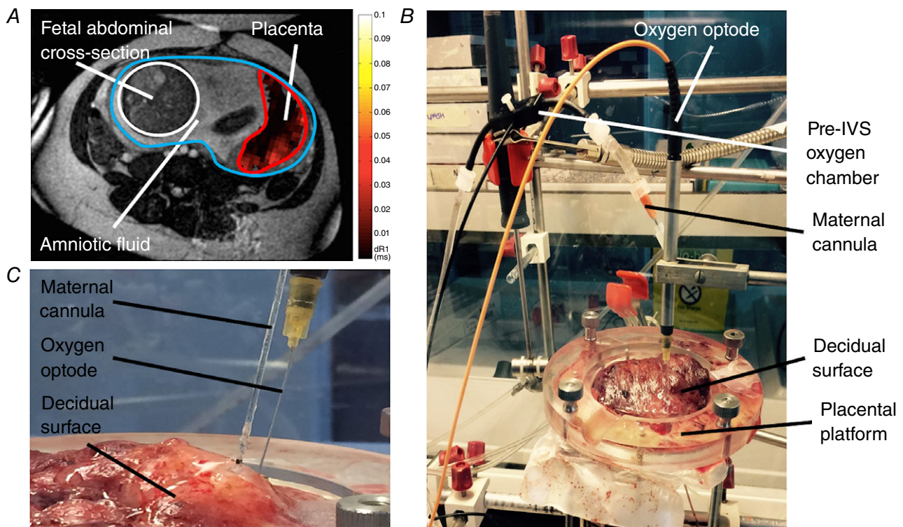
Figure 2. Measuring oxygen distribution in the human placenta
