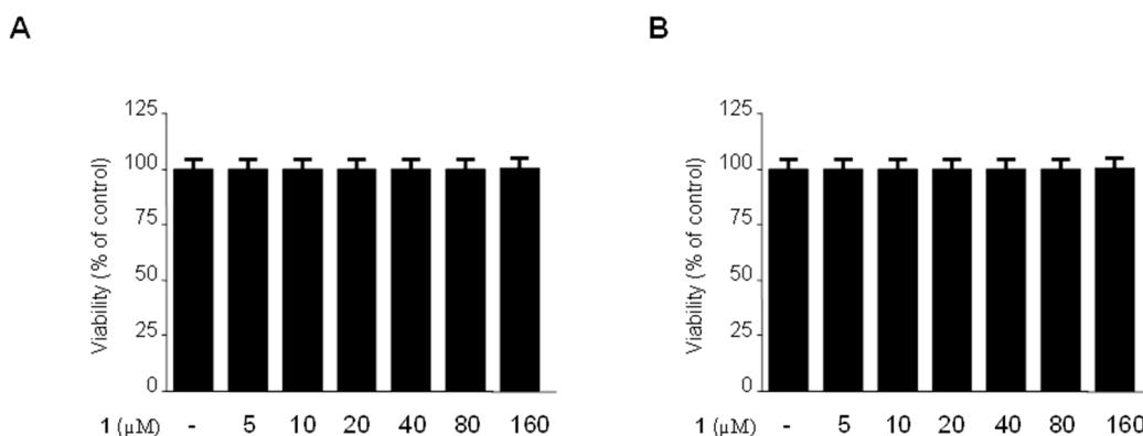
Figure 2. Effects of 1 on cell viability of RAW264.7 macrophages (A) and BV2 microglia (B). Cells were incubated for 24 h with the indicated concentrations of 1 (5–160 \mu\text{M} ). Cell viability was determined as described in Section 3.4. Data are mean \pm standard deviation (S.D.) of 3 independent experiments.
