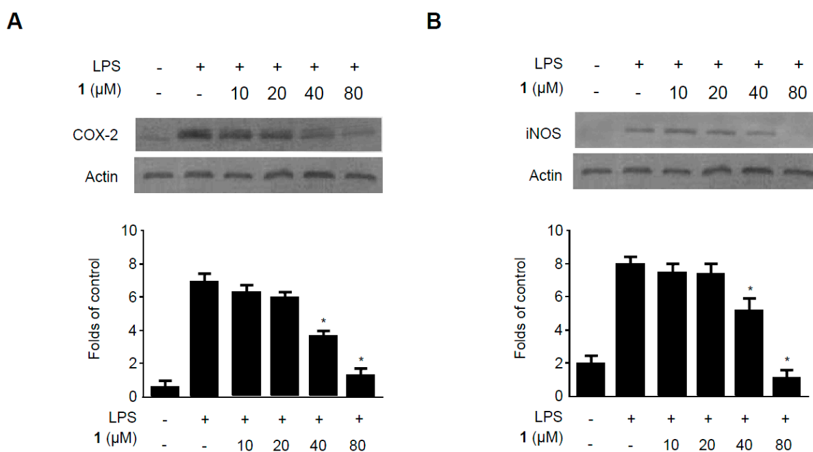
Figure 6. Effects of methylpenicinoline ( 1 ) on COX-2 (A) and iNOS (B) expression in BV2 microglia stimulated with LPS. Cells were pre-treated for 30 min with indicated concentrations of 1 and then for 24 h with LPS (500 ng/mL). Western blot analyses (A,B) were performed as described in Section 3.7; representative blots of three independent experiments are shown. Data are the mean values of three experiments \pm S.D. * p < 0.05 compared to the group treated with LPS alone.
