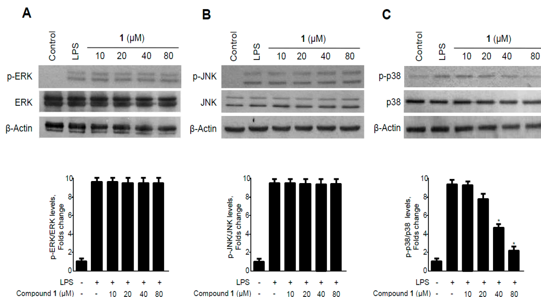
Figure 10. Effects of methylpenicillinolone ( 1 ) on ERK, JNK, and p38 MAPK phosphorylation and protein expression in BV2 microglia. Cells were pre-treated for 30 min with the indicated concentrations of 1 and stimulated for 30 min with LPS (500 ng/mL) (A–C). The levels of (A) phosphorylated-ERK (p-ERK); (B) phosphorylated-JNK (p-JNK); and (C) phosphorylated-p38 MAPK (p-p38 MAPK) were determined by western blotting. Representative blots from three independent experiments are shown. Data represent the mean values of three experiments ± S.D. * p < 0.05 compared to the group treated with LPS alone.
