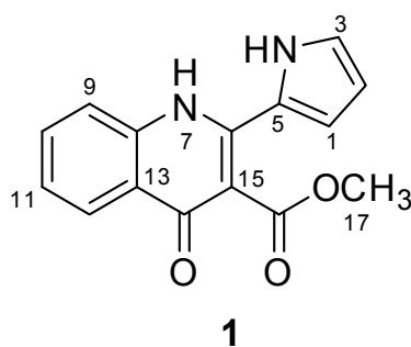
Figure 1. Chemical structure of methylpenicoline ( 1 ).
