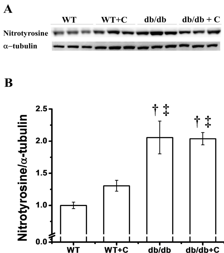
Figure 5. Effect of curcumin on the protein nitration (NT) content. (A) Representative western blot of the NT and of \alpha -tubulin in liver. (B) Densitometry analysis of the NT/ \alpha -tubulin ratio. Data are the means of n = 3 \pm SEM. ^\dagger vs. WT+C, p < 0.05 ; ^\ddagger vs. WT, p < 0.005 .
