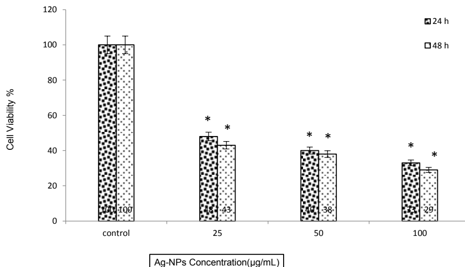
Figure 6. MTT assay results from treatment MCF-7 cell with various Ag-NPs concentration in 24 h and 48 h, Mean ± SD, * p < 0.05 .
