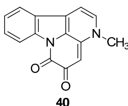
Figure 3. Structure of canthine 40.
