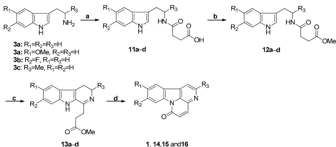
Scheme 3. The synthetic strategy of Soriano-Agaton. Reagents and conditions. (a) Succinic anhydride, DCM, RT, 18 h, 98%, 99%, 98%, and 98% for 11a–d , respectively; (b) Amberlyst 15, MeOH, reflux, 18 h, 98%; (c) POCl 3 , PhH, reflux, 1 h; (d) DBU, DCM, RT, 18 h, 80%, 70%, 80%, and 20% in two steps for 1, 14, 15, and 16 , respectively.
