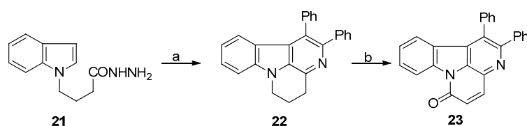
Scheme 5. The synthetic strategy of Lindsley. Reagents and conditions. (a) 1,2-Diphenylethanedione, AcONH 4 , AcOH, 220\text{ }^\circ\text{C} , 40 min, 80%; (b) 4,5-bis(thioacetamido)pentanoyl (BTAP), AcOH, 70\text{ }^\circ\text{C} , 4 h, 60%.
