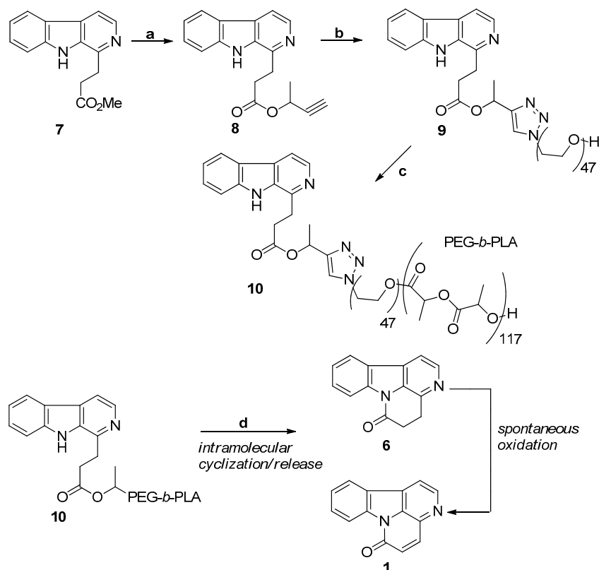
Scheme 2. The relevant biosynthetic assembly lines. Reagents and conditions: 7-functionalized nanoparticles and the biomimetic release of 1 and 6. (a) DCM, Yb(Otf) 3 (20 mol %), reflux, 16 h, 27%; (b) 3-butyn-2-ol (excess), N 3 -PEG-OH (1 equiv.), CuBr (1 equiv.), dimethylformamide, room temperature (RT), 24 h, PMDTA ( N,N,N',N'',N'' -pentamethyldiethylenetriamine), 46%; (c) d,l -lactide (excess), Sn(Oct) 2 (0.4 equiv.), toluene, 115 °C, 16 h, 57%; (d) 1,8-diazabicyclo[5.4.0]undec-7-ene (DBU) (excess), DCM, air, 72 h (identification of 1 and 6 by mass spectrometry and high-performance liquid chromatography-ultraviolet detection studies).
