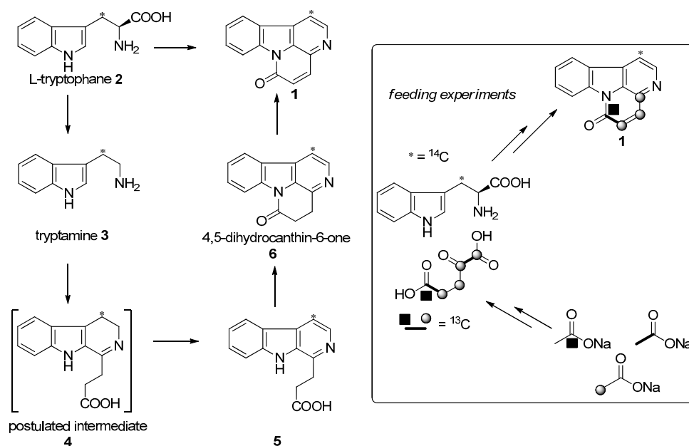
Scheme 1. Biosynthetic mechanism leading to canthin-6-one alkaloids, and the supporting feeding experiments.
