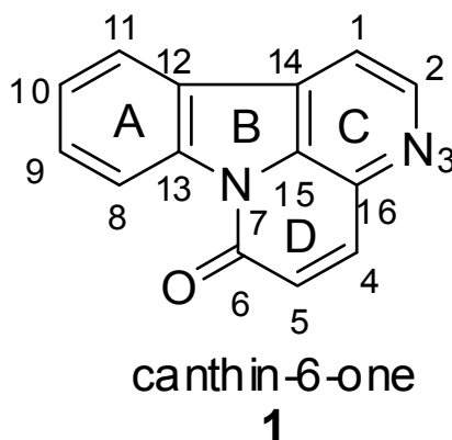
Figure 1. Structure of canthin-6-one 1.
