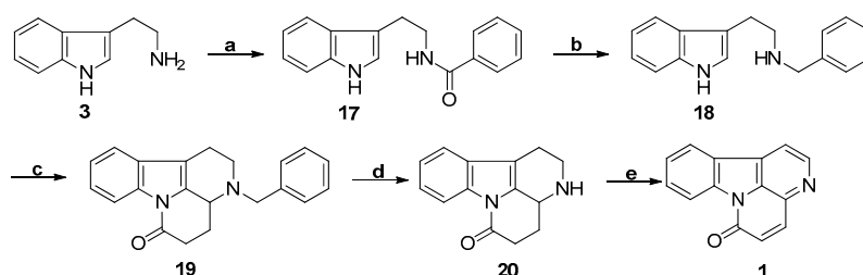
Scheme 4. The synthetic strategy of Czerwinski. Reagents and conditions. (a) Anhydrous acetone, PhCOCl, NaOH, -30\text{ }^\circ\text{C} , 95%; (b) anhydrous tetrahydrofuran (THF), LiAlH 4 , 0\text{ }^\circ\text{C} —reflux, 95%; (c) \alpha -ketoglutaric acid, PhH/dioxane (6:4), Dean-Stark trap, reflux, 80%; (d) anhydrous MeOH, Pd/C, HCOONH 4 , reflux, 83%; (e) PhH/PhMe (3:1), MnO 2 , reflux, 78%.
