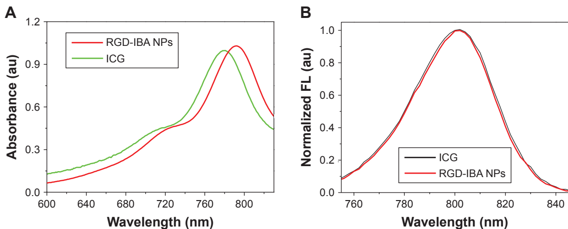
Figure 3 Spectra characterization.
