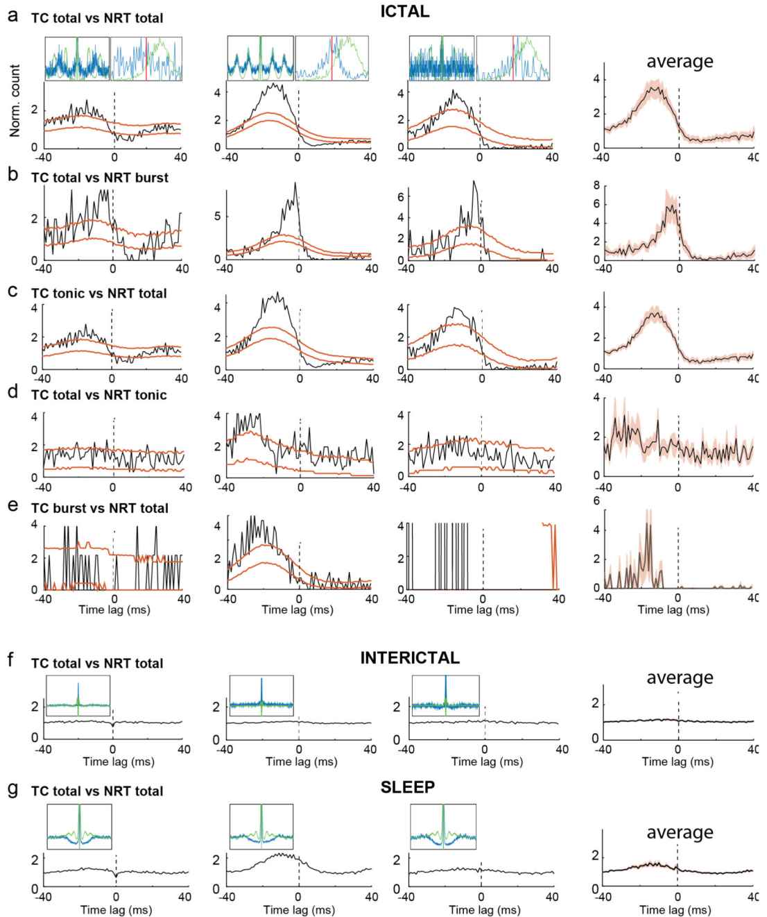
Figure 5. Ictal recruitment of NRT-TC neuron inhibitory assemblies.
