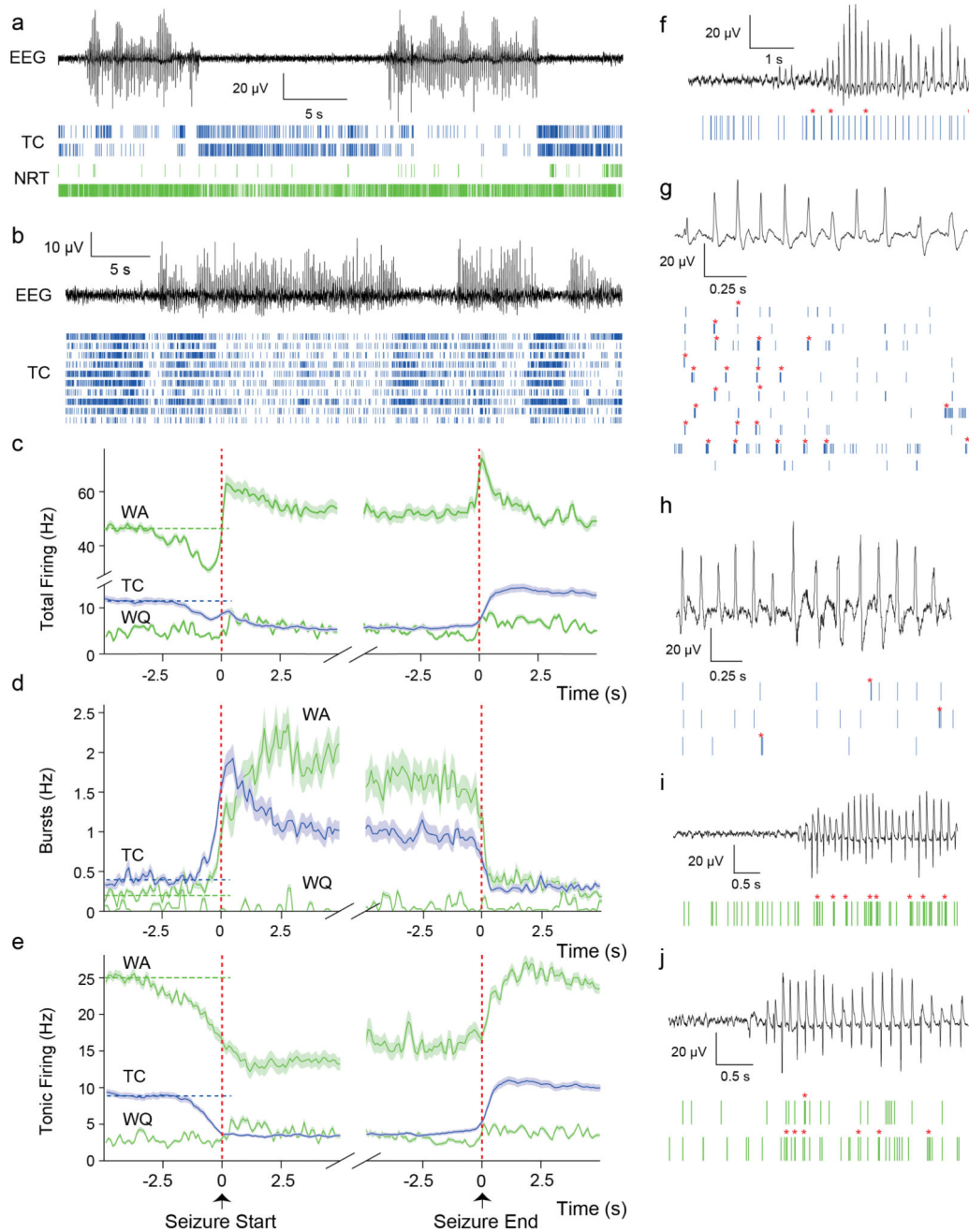
Figure 2. Temporal dynamics of TC and NRT neuron ensemble firing during ASs in GAERS.
