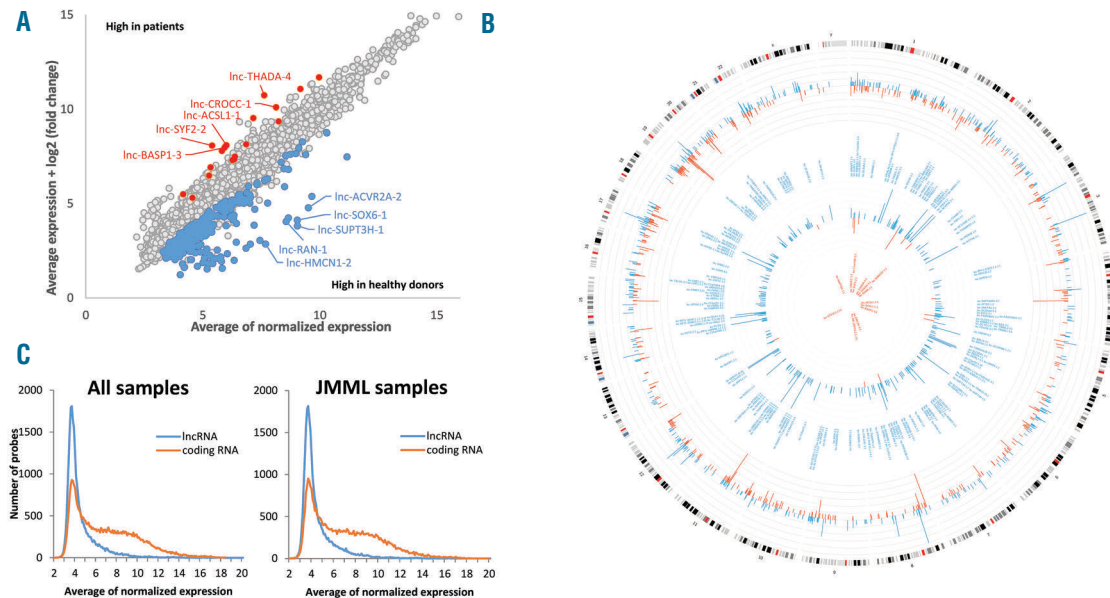
Figure 1. Long non-coding RNA transcriptome in juvenile myelomonocytic leukemia (JMML). (A) Diagonal plot representing the average expression versus the log 2 fold change added to the average expression of lncRNAs when comparing JMML (n=44) to healthy donors (n=7). lncRNAs significantly up-regulated in patients are represented in red and lncRNAs significantly down-regulated in blue. The names of the top 5 up- and down-regulated lncRNAs based on log 2 fold change are indicated. (B) Circos plot showing lncRNAs and mRNAs on human chromosomes. From the outside in, the first layer of the Circos plot represents a chromosome map of the human genome. Black and white bars are chromosome cytobands, and red bars represent centromeres. The second circle shows all differentially expressed genes when comparing JMML patients with healthy donors, and the inner circle shows all differentially expressed lncRNAs. Up-regulated lncRNA and mRNA genes are represented in red and down-regulated genes in blue. The height of the bars is representative for the fold change between JMML and healthy donors. Names of lncRNA genes with fold change of more than 2 between JMML and healthy donors are indicated between the circles with mRNA and lncRNA genes for the down-regulated lncRNAs and in the middle of the plot for the up-regulated lncRNAs. (C) Density plots representing the average of the normalized expression of all lncRNAs and mRNAs detected by the array in all samples (left) and in JMML samples only (right).
