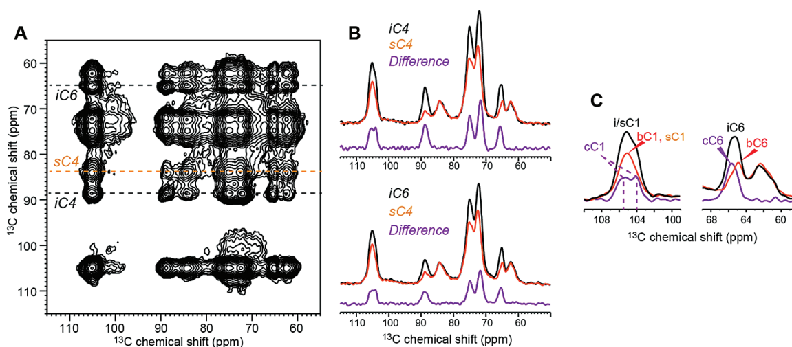
Fig. 4. 2D ^{13}\text{C} - ^{13}\text{C} PDSD spectrum of Arabidopsis cell walls with a 1.5 s mixing time. The spectrum was measured at -20^\circ\text{C} under 9 kHz MAS. (A) 2D spectrum. (B) Representative cellulose cross sections of interior and surface cellulose exhibit different intensity patterns. The difference spectra (purple) were obtained after normalizing the two spectra by the sC4 peak. The surface cellulose cross section has contribution from Ara and XyG backbone, but the difference spectra mainly show signals of interior cellulose. (C) C1 and C6 regions of the cellulose cross sections and the difference spectra. Core cellulose C1 shows two peaks at 105.5 ppm and 104.1 ppm, and core cellulose C6 (cC6) exhibits a 0.3 ppm downfield shift from the average interior cellulose C6 (iC6) and 0.6 ppm downfield shift from the surface-bound interior cellulose (bC6).
