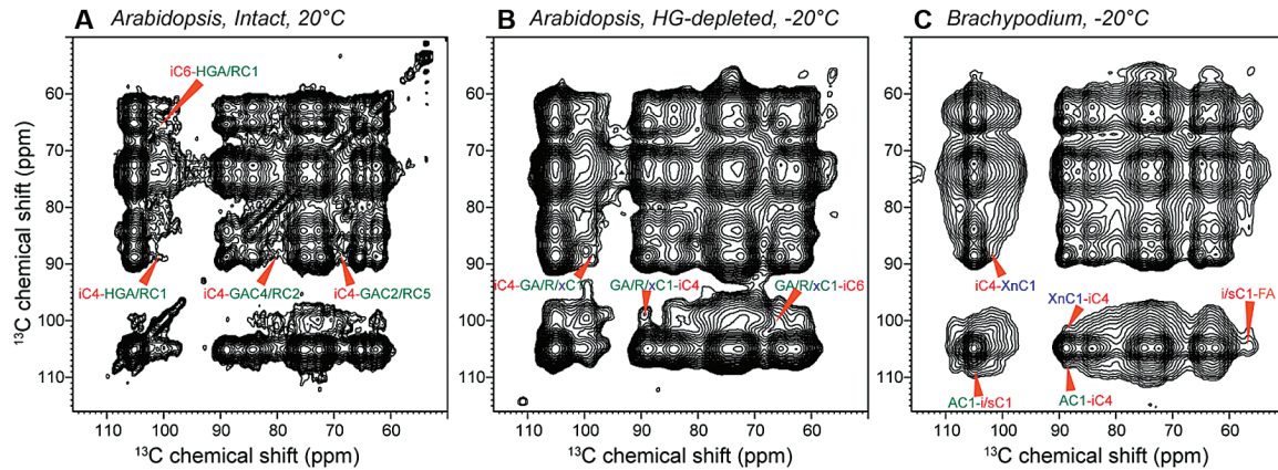
Fig. 2. 2D ^{13}\text{C} - ^{13}\text{C} PDS spectra of plant cell walls measured with 1.5 s spin diffusion mixing. (A) Intact Arabidopsis cell wall at 20 °C. (B) HG-depleted Arabidopsis cell wall at -20 °C. (C) Brachypodium cell wall at -20 °C. Cellulose–pectin cross peaks are observed in both intact and HG-depleted Arabidopsis cell walls, and cellulose–GAX cross peaks are detected in the Brachypodium sample.
