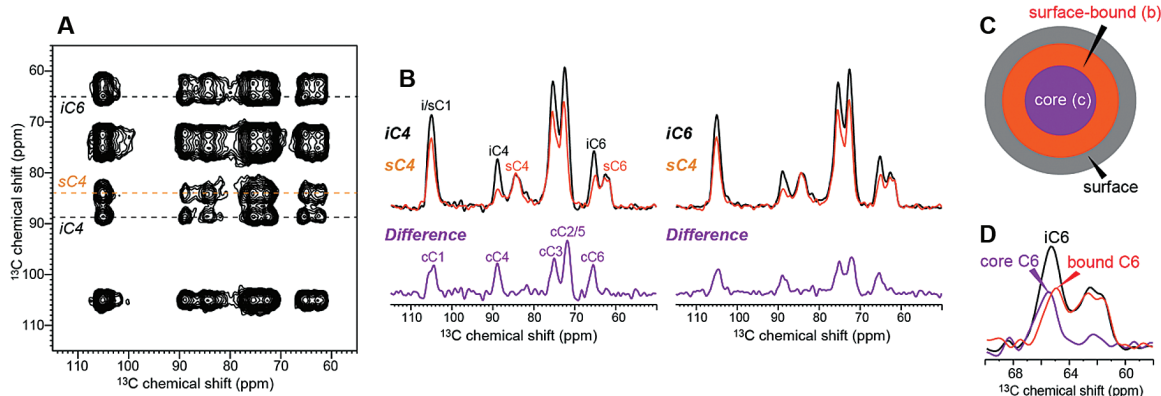
Fig. 3. (A) 2D ^{13}\text{C} - ^{13}\text{C} PDSM spectrum of Brachypodium cell wall with a 3.0 s mixing. The spectrum was measured at 20 °C with a short ^1\text{H} - ^{13}\text{C} CP contact time of 35 \mu\text{s} to suppress the signals of mobile GAX. (B) Representative cross sections of interior cellulose (black) and surface cellulose (orange). The different intensity patterns indicate that ^{13}\text{C} magnetization has not equilibrated between interior and surface cellulose. The difference spectra (purple), obtained after normalizing the two cross sections by the sC4 peak, correspond to core cellulose chains that are inaccessible to the surface. (C) Illustration of the cellulose microfibril structure, where interior cellulose consists of a surface-bound fraction and a core fraction. (D) The two types of interior cellulose chains have slightly different C6 chemical shifts.
