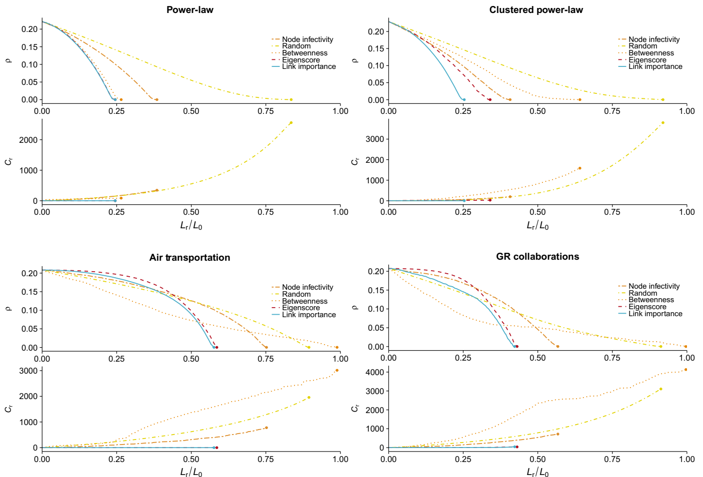
Fig. 2. Targeted bond percolation. We show the incidence of the epidemics, ( \rho ), and the number of connected components, ( C_r ), as functions of the occupation probability, ( L_r/L_0 ), where L_0 is the number of links of the network and L_r is the number of removed edges in the bond percolation process. We compare five different epidemic containment strategies: removing the edges of the node with the highest probability of being infected, P(\sigma_i = I) (orange dash-dash lines); a random edge removal (yellow dash-dot lines); removing the edge with the highest edge betweenness (light orange dotted lines); targeting the edge with the highest eigenscore (red dashed line); and, last, removing the edge that has the largest link epidemic importance (blue solid line). We apply these processes to the same networks as in Fig. 1 (see Methods). We have set the recovery rate to \mu = 0.5 and have chosen the infection probability \beta such that the stationary incidence of the epidemics is about \rho_{ini} \approx 0.2 for all the networks, that is, \beta = 0.1 for both power-law networks, \beta = 0.06 for air transportation network, and \beta = 0.11 for the collaboration network. The dots mark the achievement of total containment.
