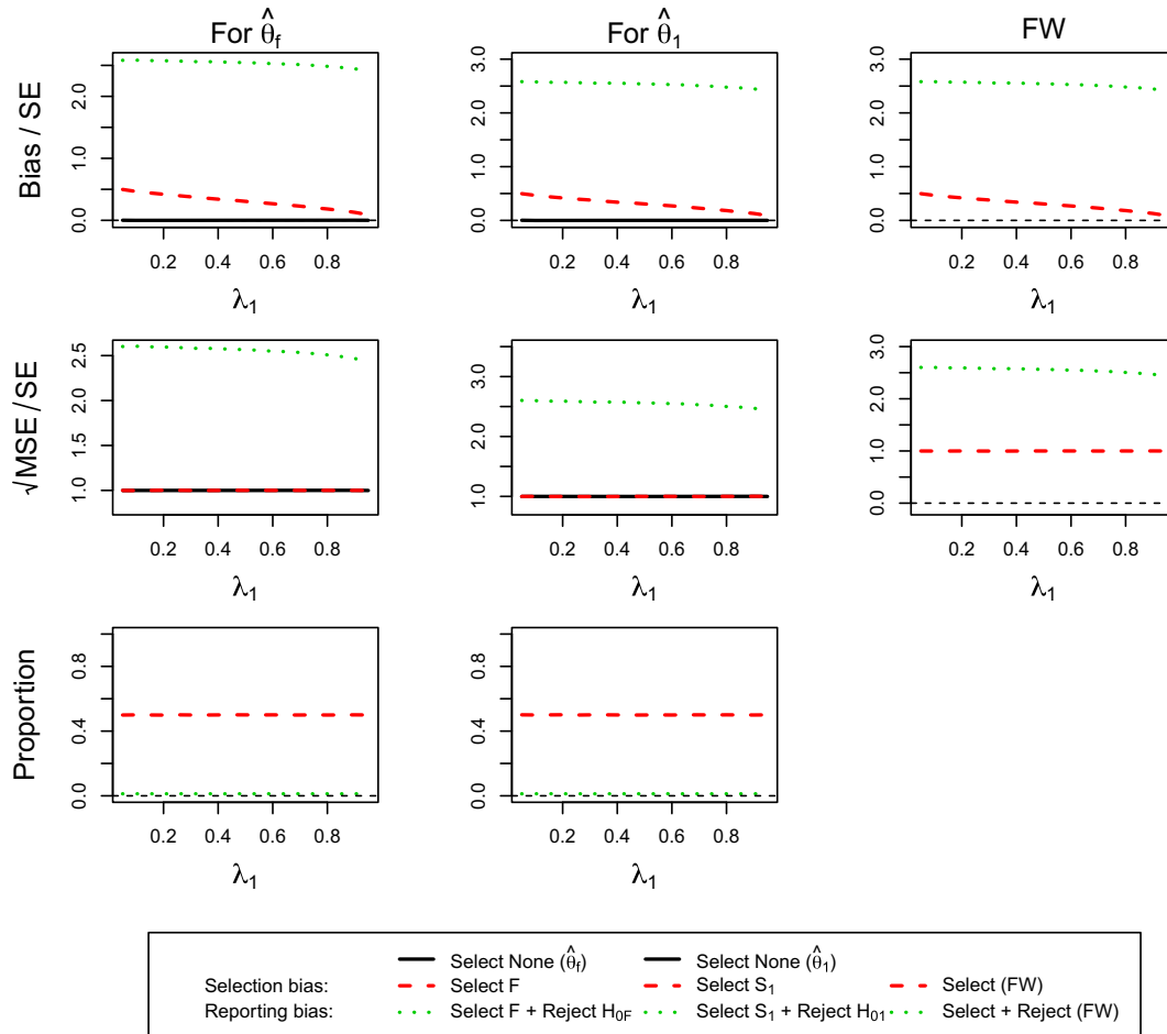
FIGURE 2 (For Design 1 , \theta_1 = 0 , and \theta_2 = 0 ) the standardized bias and standardized \sqrt{\text{MSE}} of maximum likelihood estimators \hat{\theta}_f, \hat{\theta}_1 and the simulation proportions for different circumstances against the prevalence of subpopulation 1, ie, \lambda_1 . FW, family-wise; MSE, mean squared error [Colour figure can be viewed at wileyonlinelibrary.com ]
