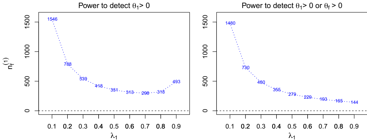
FIGURE 1 The total sample sizes of the full population F(n_f^{(1)}) across prevalence rates of S_1 ( \lambda_1 ) for two different definitions of power. The design is a single-stage design with two subpopulations where the treatment effects \theta_1 and \theta_2 for S_1 and S_2 are 0.5 and 0, respectively. The type-I error and power are specified at 0.025 and 80% [Colour figure can be viewed at wileyonlinelibrary.com ]
