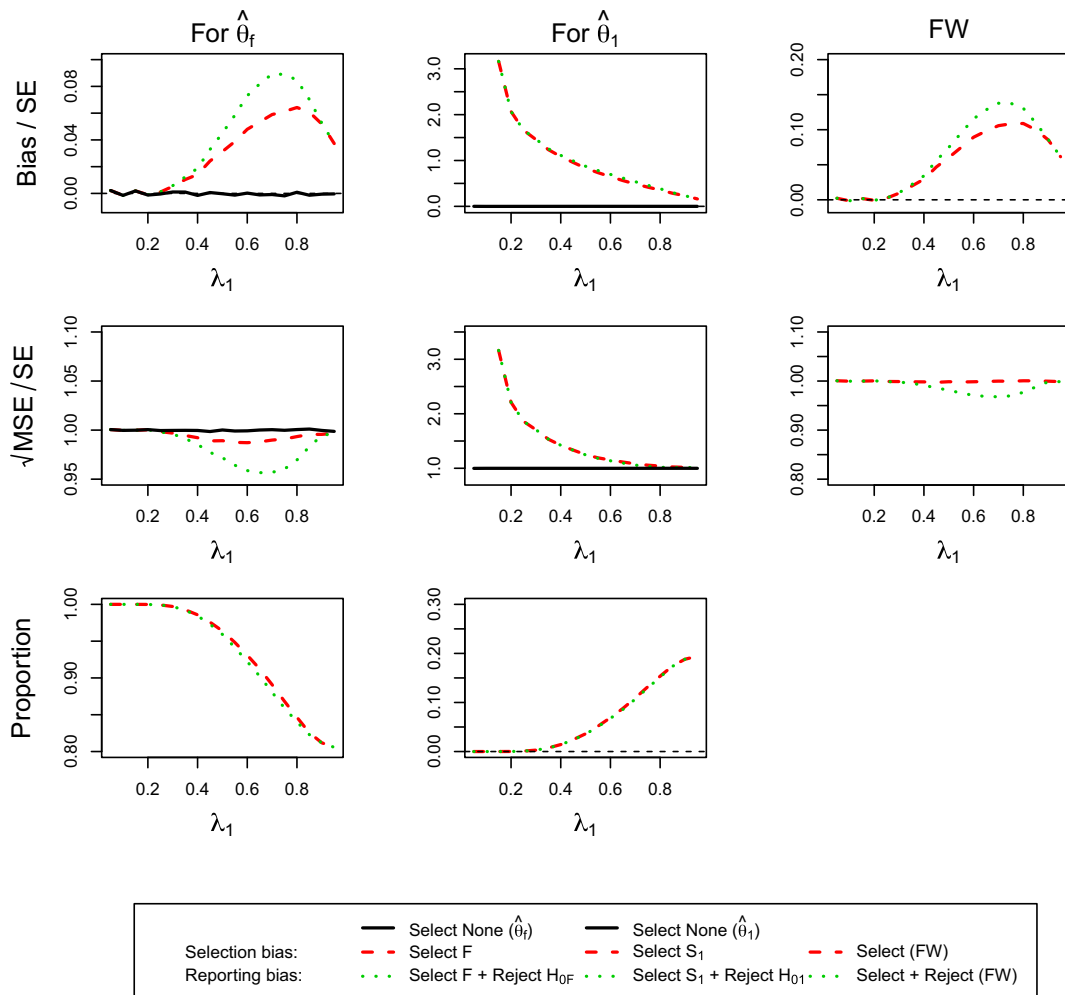
FIGURE 4 (For Design 1 , \theta_1 = 0.5 and \theta_2 = 0.5 ) the standardized bias and standardized \sqrt{\text{MSE}} of maximum likelihood estimators \hat{\theta}_f , \hat{\theta}_1 and the simulation proportions for different circumstances against the prevalence of subpopulation 1, ie, \lambda_1 . FW, family-wise; MSE, mean squared error [Colour figure can be viewed at wileyonlinelibrary.com ]
