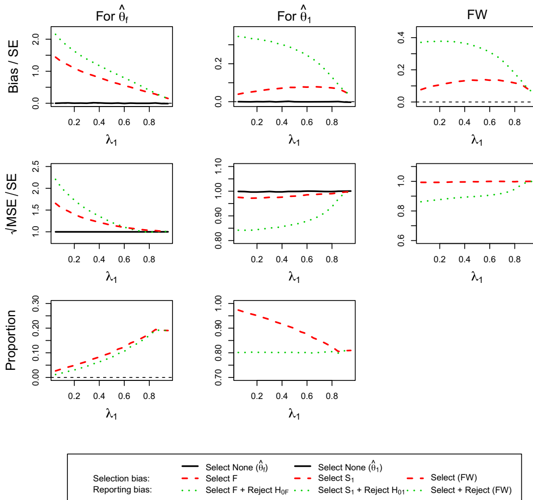
FIGURE 3 (For Design 1 , \theta_1 = 0.5 and \theta_2 = 0 ) the standardized bias and standardized \sqrt{\text{MSE}} of maximum likelihood estimators \hat{\theta}_f, \hat{\theta}_1 and the simulation proportions for different circumstances against the prevalence of subpopulation 1, \lambda_1 . FW, family-wise; MSE, mean squared error [Colour figure can be viewed at wileyonlinelibrary.com ]
