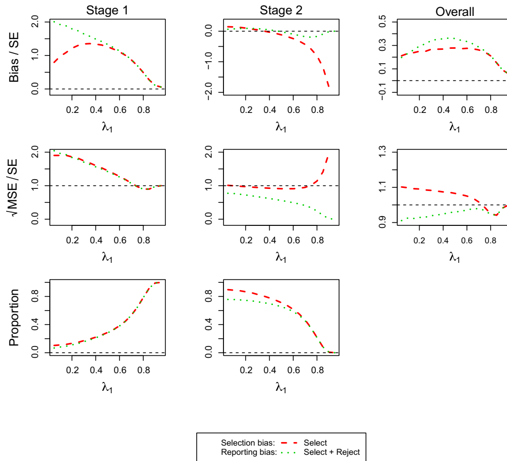
FIGURE 7 (For Design 3 , \theta_1 = 0.5 and \theta_2 = 0 ) FW bias and mean squared error and simulation proportions for different circumstances at stopping stage 1, 2, and overall, against the prevalence of subpopulation 1, ie, \lambda_1 [Colour figure can be viewed at wileyonlinelibrary.com]
