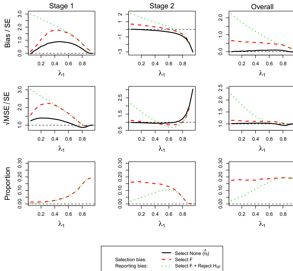
FIGURE 5 (For Design 3 , \theta_1 = 0.5 and \theta_2 = 0 ) standardized bias and mean squared error (MSE) of \hat{\theta}_f and simulation proportions for different circumstances at stopping stage 1, 2, and overall, against the prevalence of subpopulation 1, ie, \lambda_1 [Colour figure can be viewed at wileyonlinelibrary.com]
