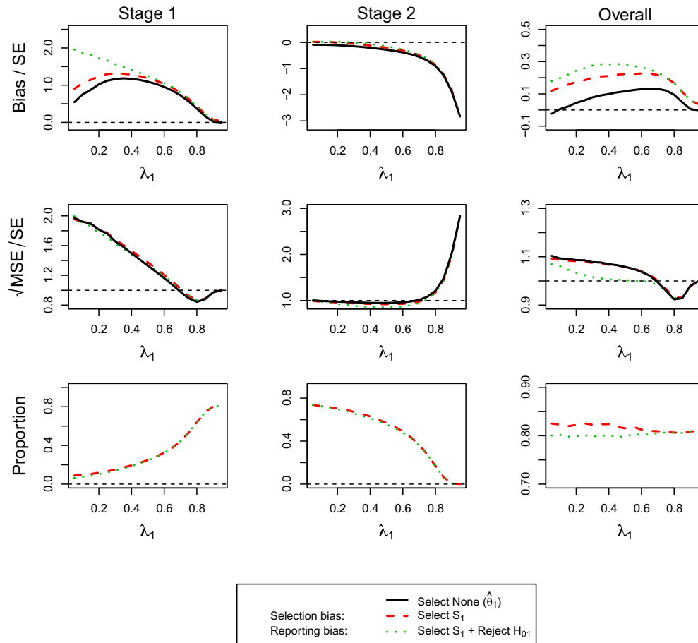
FIGURE 6 (For Design 3 , \theta_1 = 0.5 and \theta_2 = 0 ) standardized bias and mean squared error (MSE) of \hat{\theta}_1 and simulation proportions for different circumstances at stopping stage 1, 2, and overall, against the prevalence of subpopulation 1, ie, \lambda_1 [Colour figure can be viewed at wileyonlinelibrary.com]
