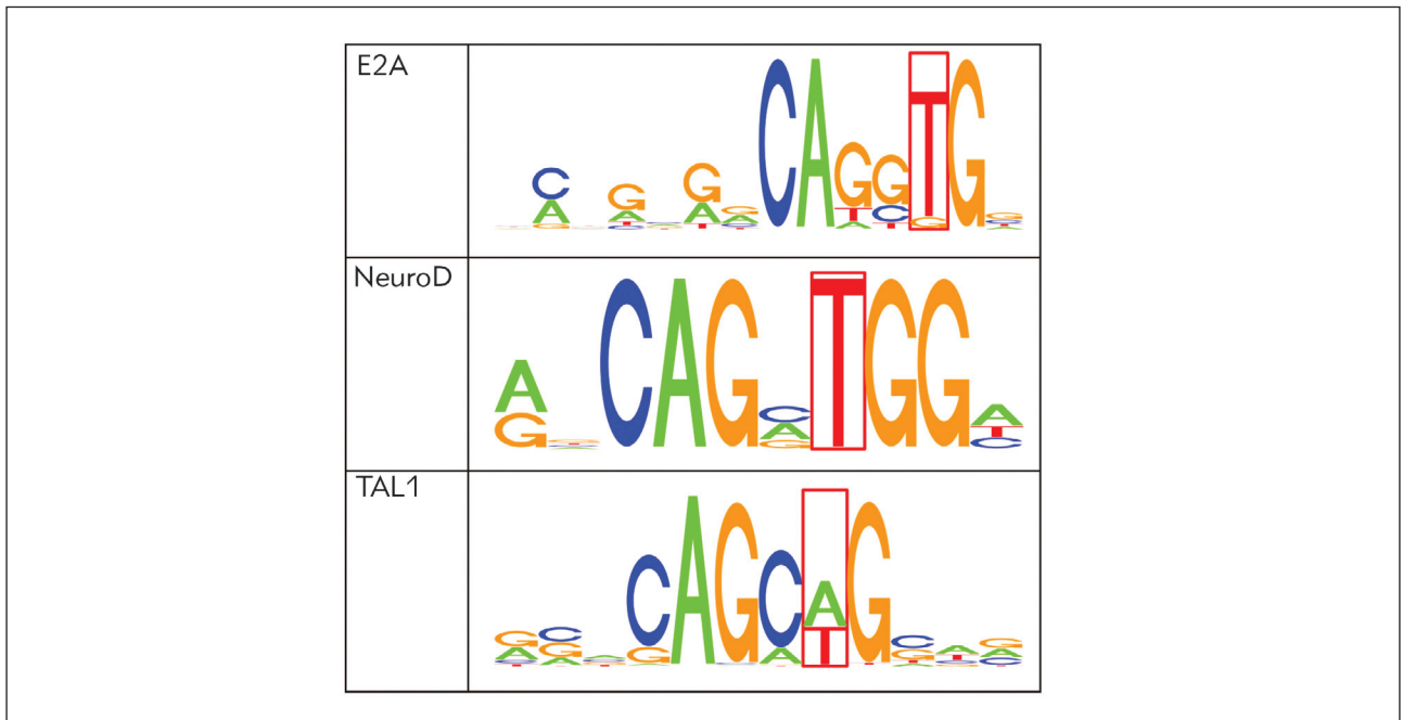
Figure 2 Canonical motif for E2A, NeuroD and TAL1 transcriptional factors.
