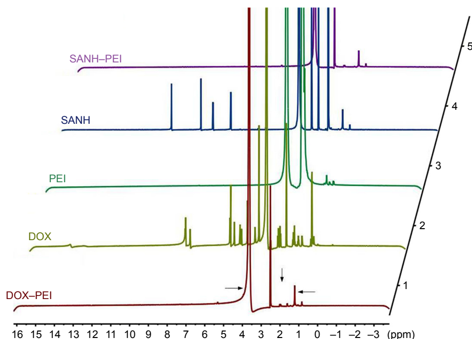
Figure 2 The ^1\text{H} NMR spectrum of PEI, SANH, SANH-PEI, DOX, DOX-PEI.
