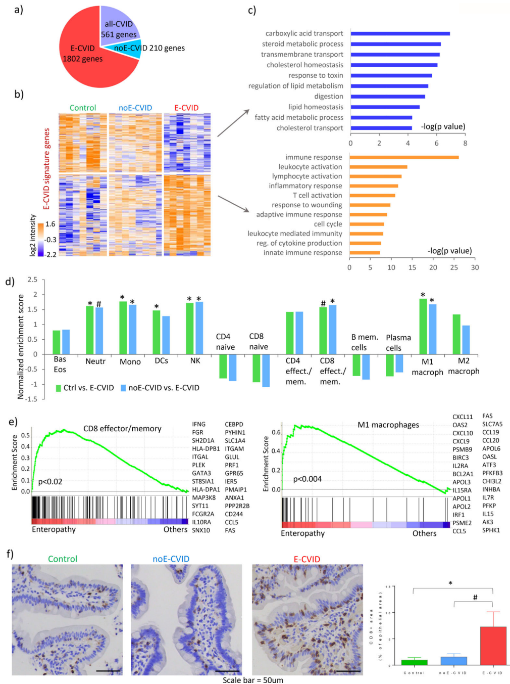
Figure 1. Gene expression and cellular characterization of CVID enteropathy. (a) Number of genes assigned to each of the three signatures (E-CVID, noE-CVID and all-CVID) defined as described in Methods and Supplementary Figure 1. (b) heatmap of genes in E-CVID profile; columns, samples (Control n=7, noE-CVID n=8, E-CVID n=7), rows, genes; log 2 normalized intensities of gene expression across all samples are represented. (c) Enriched Gene Ontology terms (Biological Process) in E-CVID profile (p-values obtained using DAVID bioinformatics resources). (d) Gene set enrichment analysis (GSEA) for
