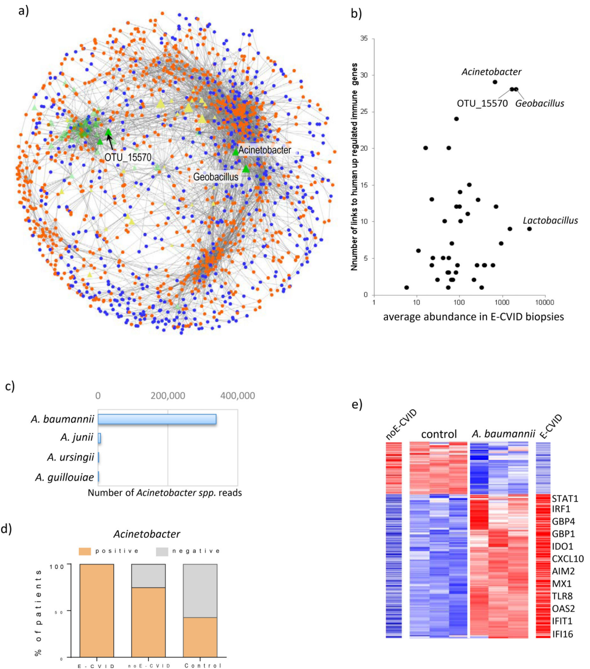
Figure 4. Transkingdom network analysis identifies Acinetobacter baumannii as a candidate microbe driving CVID enteropathy. (a) Transkingdom network reconstructed from levels of expression of human genes from E-CVID signature and candidate microbes selected based on analysis in Fig. 3d; orange and blue indicate up-regulated and downregulated genes in E-CVID, respectively; green and yellow are bacterial OTUs increased or decreased in E-CVID, respectively. (b) Number of connections to genes up-regulated in E-CVID and average abundance in E-CVID biopsies are plotted for each OTU identified by analysis in Fig. 3d.
