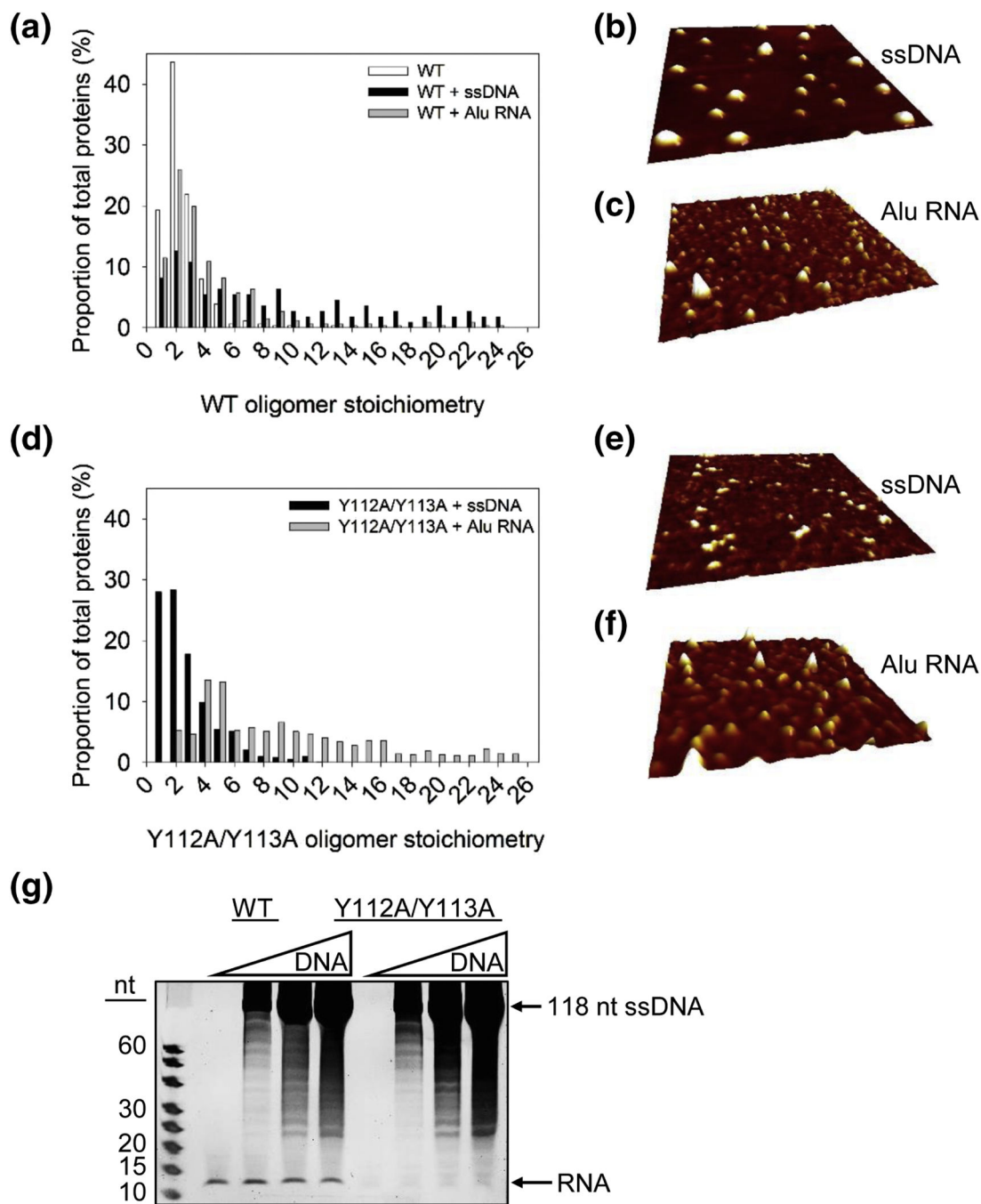
Figure 5. Oligomerization states of A3H on ssDNA and Alu RNA. (A-F) AFM imaging was done in the presence of 5 mM MgCl 2 . (A-C) The oligomeric state of A3H WT alone (WT) and bound to ssDNA (WT + ssDNA) or Alu RNA (WT + Alu RNA) demonstrated that oligomerization predominantly occurred on ssDNA. (D-F) A3H Y112A/Y113A bound to ssDNA (Y112A/Y113A + ssDNA) or Alu RNA (Y112A/Y113A + Alu RNA) demonstrated that oligomerization predominantly occurred on Alu RNA. Volume distributions of A3H were converted to stoichiometries based on analysis of dimeric A3H WT (WT).
