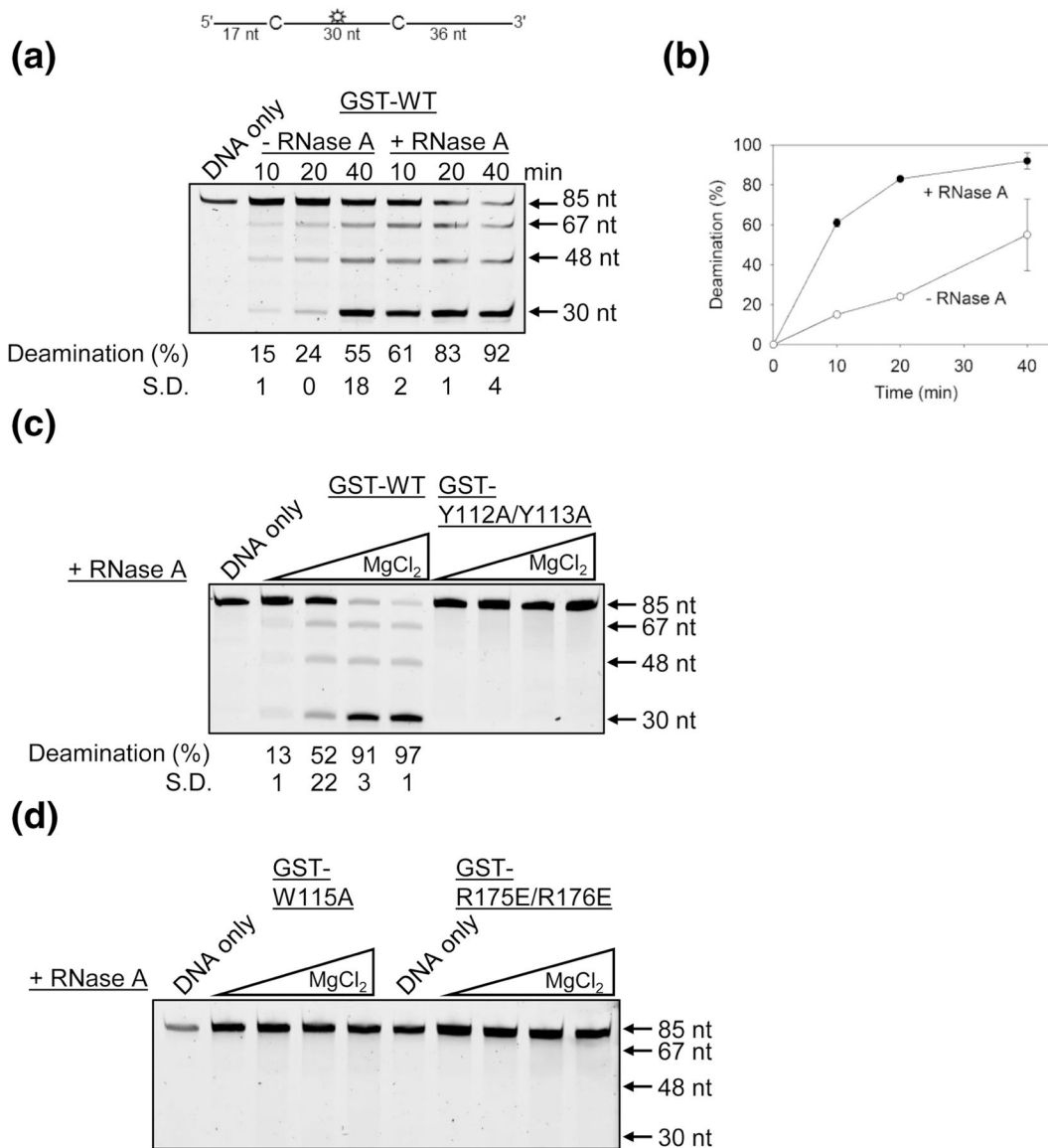
Figure 2. Deamination of ssDNA by GST-A3H. Deamination activity was tested on an 85 nt ssDNA with two 5' CTC deamination motifs separated by 30 nt. (A-B) A3H WT can deaminate ssDNA in the presence and absence of bound cellular RNA. (C-D) Monomeric A3H mutants have disrupted ssDNA deaminase activity. Using different MgCl 2 concentrations that were found to enhance GST-A3H WT activity, the deamination activity of A3H mutants were tested in the presence of RNase A. (C-D) The A3H GST-Y112A/, GST-W115A and GST-R175E/R176E were not active on ssDNA. A representative image is shown from three independent experiments. The S.D. was calculated from three independent experiments and is shown below the gel or for panel (B) is represented by error bars. Some error bars in (B) are obscured by the symbol.
