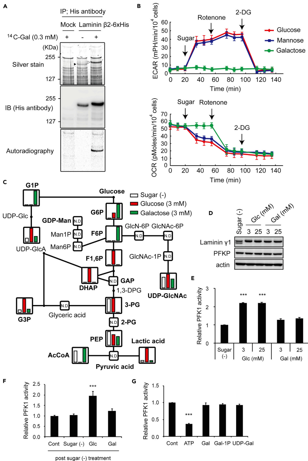
Figure 3. Alteration of Metabolism in Response to Galactose
