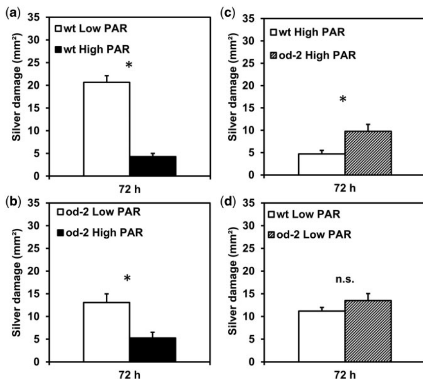
Fig. 2 Feeding preference of the Western flower thrips F. occidentalis for low and high PAR-treated wild-type (wt) and odorless-2 ( od-2 ) plants tested in leaf disc dual-choice bioassays. Leaf discs were taken from leaflets belonging to the third/fourth youngest leaf at 35 d after initial light treatments. Silver damage (mean \pm SEM, n = 25-30 ) caused by thrips feeding was evaluated at 72 h after thrips release in the following pair-wise comparisons: (a) low PAR vs. high PAR-treated wild-type plants; (b) low PAR vs. high PAR-treated od-2 plants; (c) high PAR-treated wild-type vs. high PAR-treated od-2 plants; and (d) low PAR-treated wild-type vs. low PAR-treated od-2 plants. Pooled data from three independent experiments were analyzed. Asterisks denote significant differences tested by Wilcoxon signed rank test ( P \leq 0.05 ). n.s. = not significant.
