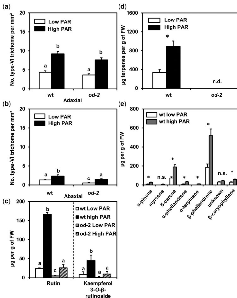
Fig. 3 Effect of low and high PAR treatments on type VI leaf trichome-associated defenses in wild-type (wt) and odorless-2 ( od-2 ) plants. Type VI trichome density was evaluated on (a) adaxial and (b) abaxial leaf sides of leaflets taken from the third/fourth youngest leaf at 35 d after initial light treatments. Values represent the mean ( \pm SEM) of 28–29 plants from three independent experiments. (c) Main phenolic compounds identified in leaf exudates of low or high PAR-treated wild-type and od-2 plants. Values represent the mean ( \pm SEM) of nine plants from two independent experiments. (d) Total terpene content (mean \pm SEM, n = 4-5 ) measured in leaf exudates of leaflets taken from the third/fourth youngest leaf and (e) levels (mean \pm SEM, n = 4-5 ) of individual terpene compounds. Asterisks denote significant differences between low and high PAR-treated wild-type plants analyzed by t -test or Mann–Whitney U tests ( P \leq 0.05 ). Different letters above bars denote significant differences among groups (ANOVA followed by Fisher's LSD test, P \leq 0.05 ). n.s. = not significant. n.d. = not detected.
