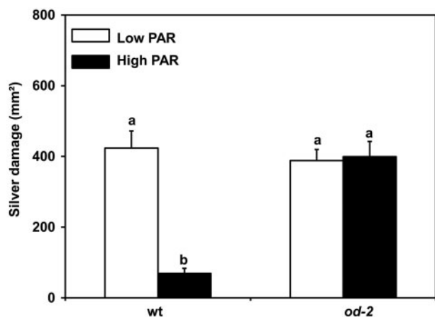
Fig. 1 Effect of low and high PAR treatments on tomato resistance to the Western flower thrips F. occidentalis , tested in a whole plant no-choice bioassay, at 35 d after initial light treatments. Silver damage caused by thrips feeding was measured in low and high PAR-treated wild-type (wt) and odorless-2 ( od-2 ) plants at 12 d after thrips infestation. Values represent the mean ( \pm SEM) of 26 plants from three independent experiments. Different letters above bars denote significant differences among groups (ANOVA followed by Fisher's LSD test, P \leq 0.05 ).
