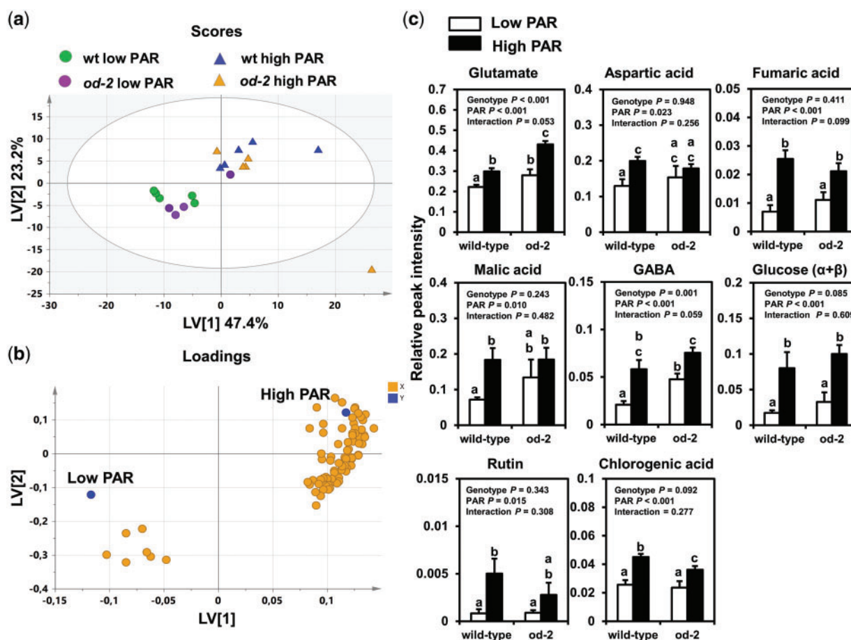
Fig. 5 Metabolomic responses in wild-type (wt) and odorless-2 ( od-2 ) plants under low or high PAR conditions. Leaf metabolites were analyzed by NMR at 35 d after initial light treatments on leaflets collected from the third/fourth youngest leaf. Projection to latent structures-discriminant analysis (PLS-DA) was performed on the obtained ^1\text{H} NMR spectra, and resulted in three latent variables (LVs) that cumulatively explained 82% of the total metabolomic variation and 84.6% of the light treatment response, with a 76.3% total model predictability. (a) Score plot showing the first two LVs. (b) Loading plot showing metabolites contributing most to the model (VIP score >1). (c) Relative spectral intensities (mean \pm SEM, n = 4-5 ), scaled to the internal standard, of selected metabolites (VIP score >1) identified in the ^1\text{H} NMR spectra. Different letters above bars denote significant differences among groups (ANOVA followed by Fisher's LSD test, P \leq 0.05 ).
