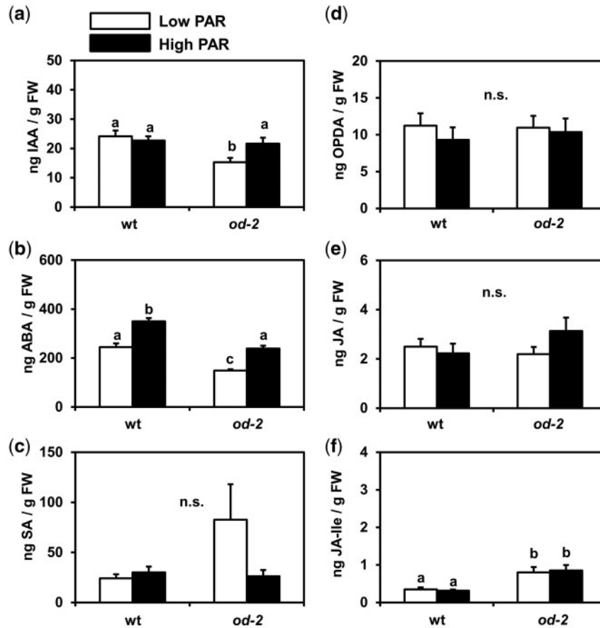
Fig. 6 Concentrations of (a) IAA, (b) ABA, (c) salicylic acid (SA), (d) 12-oxo-phytodienoic acid (OPDA), (e) jasmonic acid (JA) and (f) jasmonic acid-isoleucine (JA-Ile) determined in low and high PAR-treated wild-type (wt) and odorless-2 ( od-2 ) plants at 35 d after the initial light treatments. The analysis was performed on leaflets collected from the third/fourth youngest leaf. Values represent the mean ( \pm SEM) of five individual plants. Different letters above bars denote significant differences among groups (ANOVA followed by Fisher's LSD test, P \leq 0.05 ). n.s. not significant.
