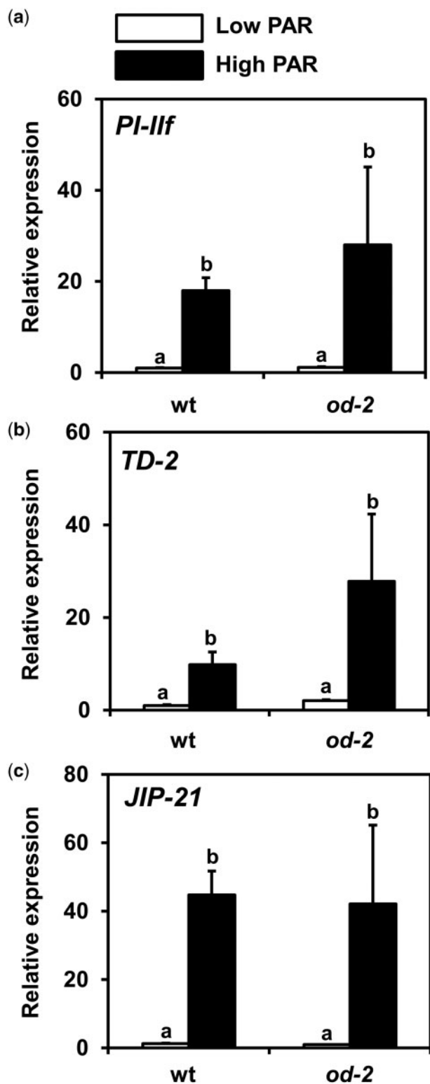
Fig. 7 Relative transcript levels of the JA-responsive genes (a) proteinase inhibitor-Ilf ( PI-Ilf ), (b) threonine deaminase-2 ( TD-2 ) and (c) jasmonate inducible protein-21 ( JIP-21 ) measured in low and high PAR-treated wild-type (wt) and odorless-2 ( od-2 ) plants at 35 d after the initial light treatment. The analysis was performed on leaflets collected from the third/fourth youngest leaf. Values represent the mean ( \pm SEM) of relative expression of each treatment group ( n = 5 biological replicates, two technical replicates). Different letters above bars denote significant differences among groups (ANOVA followed by Fisher's LSD test, at P \leq 0.05 ).
