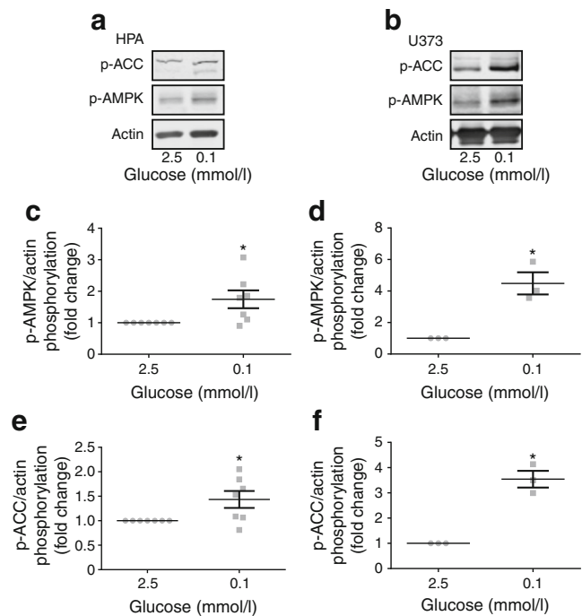
Fig. 1 Acute low glucose increased AMPK pathway activation. Representative immunoblots from HPA (a; n = 8 ) and U373 astrocytoma cells (b; n = 3 ) exposed to 2.5 or 0.1 mmol/l glucose media for 30 min. (c, d) Densitometric analysis of immunostaining for pT172 AMPK normalised to actin as a loading control in HPA (c) and U373 astrocytoma cells (d). (e, f) Densitometric analysis of immunostaining for pS79 ACC normalised to actin as a loading control in HPA (e) and U373 astrocytoma cells (f). Error bars represent SEM. *p < 0.05 , one-sample t test vs control (2.5 mmol/l glucose)
