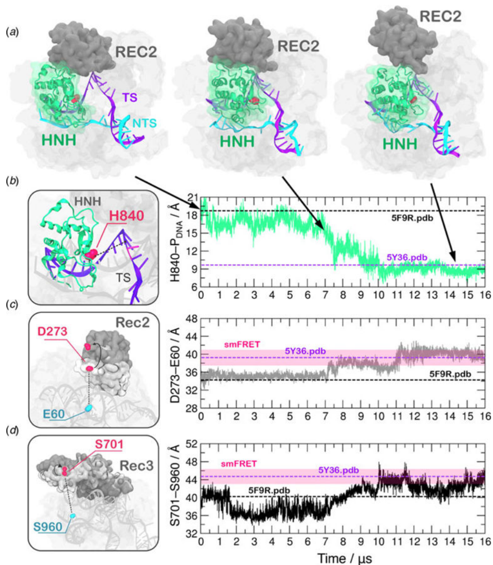
Fig. 2. (a) Conformational change of the HNH domain and structural adaptation of REC2 during ~16 \mu s of continuous MD simulations. (b–d) Time evolution along MD of: (b) the distance between H840 Ca and the scissile phosphate on the target DNA strand (phosphate at position -3), indicating the approach of the HNH domain at the cleavage site; (c) the distance between Ca atoms of E60 and D273 indicating the outward translation of REC2; (d) the distance between Ca atoms of S960 and S701 indicating the conformational change of REC3. Horizontal bars are used to indicate the value of the three distances in the X-ray structure of the pre-activated state (5F9R.pdb, starting configuration for MD) and in the model structure obtained via cryo-EM fitting of the EMD-8236 map (5Y36.pdb) (Huai et al. , 2017; Jiang et al. , 2016). Transparent boxes are used to indicate the range assumed by the distances in single molecule Förster Resonance Energy Transfer (smFRET) experiments (Chen et al. , 2017; Dagdas et al. , 2017).
