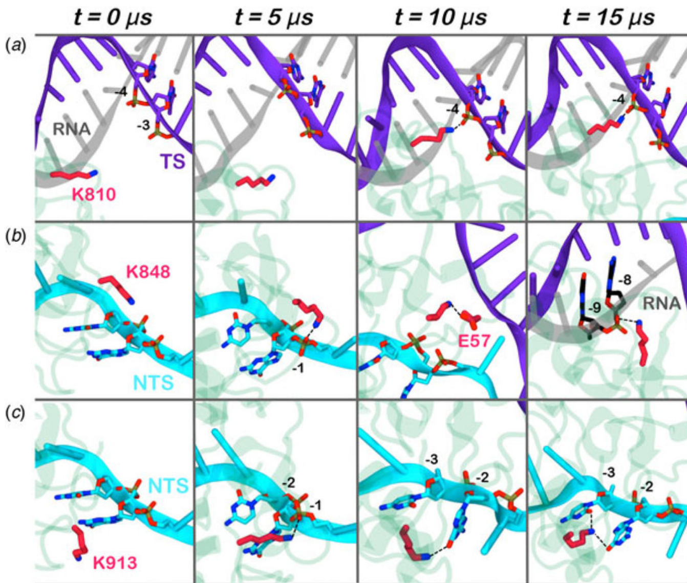
Fig. 4. Interaction established by the K810 (a), K848 (b), and K913 (c) residues of the HNH domain at ~0, 5, 10, 15 \mu s of MD. The RNA (gray), target DNA (TS, magenta), and non-target DNA (NTS, cyan) strands are shown as ribbons. The HNH domain (green) is shown as cartoon. Interacting residues are shown as sticks.
