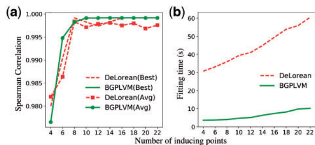
Fig. 1. Arabidopsis thaliana microarray data (Windram et al., 2012): A comparison of performance and fitting time between the proposed method and the DeLorean method. (a) Spearman correlation between the actual capture time and the estimated pseudotime for different number of inducing points. (b) Fitting time required by the models for the same experimental setups
