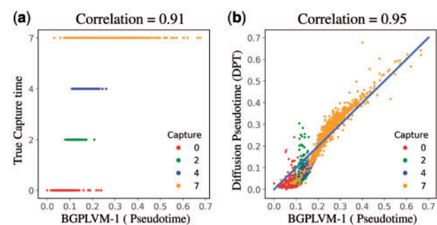
Fig. 3. Mouse embryonic stem cells (Klein et al. , 2015): Comparison of estimated pseudotime with the actual cell capture time and the pseudotime estimated using DPT. The points are coloured according to the actual cell capture times. The rank correlation is shown in the caption of each subplot (Color version of this figure is available at Bioinformatics online.)
