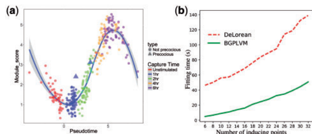
Fig. 2. Mouse dendritic cells (Shalek et al. , 2014): (a) The module score of core antiviral cells over pseudotime. The two precocious cells (plotted as triangles) have been placed in later pseudotimes than the other cells captured at 1 h. A Loess curve (solid blue line) has been plotted through the data. (b) Comparison of fitting time required by both the DeLorean and our models for different number of inducing points while using the same experimental setups (Color version of this figure is available at Bioinformatics online.)
