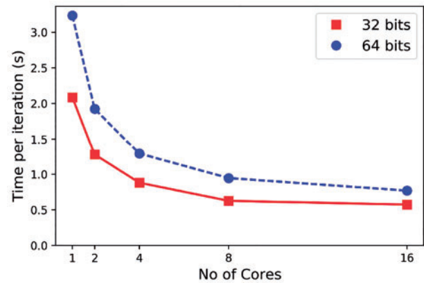
Fig. 4. PBMCs with \sim 68 k cells (Zheng et al., 2017): Time per iteration using 1, 2, 4, 8 and 16 CPU cores. The algorithm has been applied using both 32 and 64 bit floating point precision
