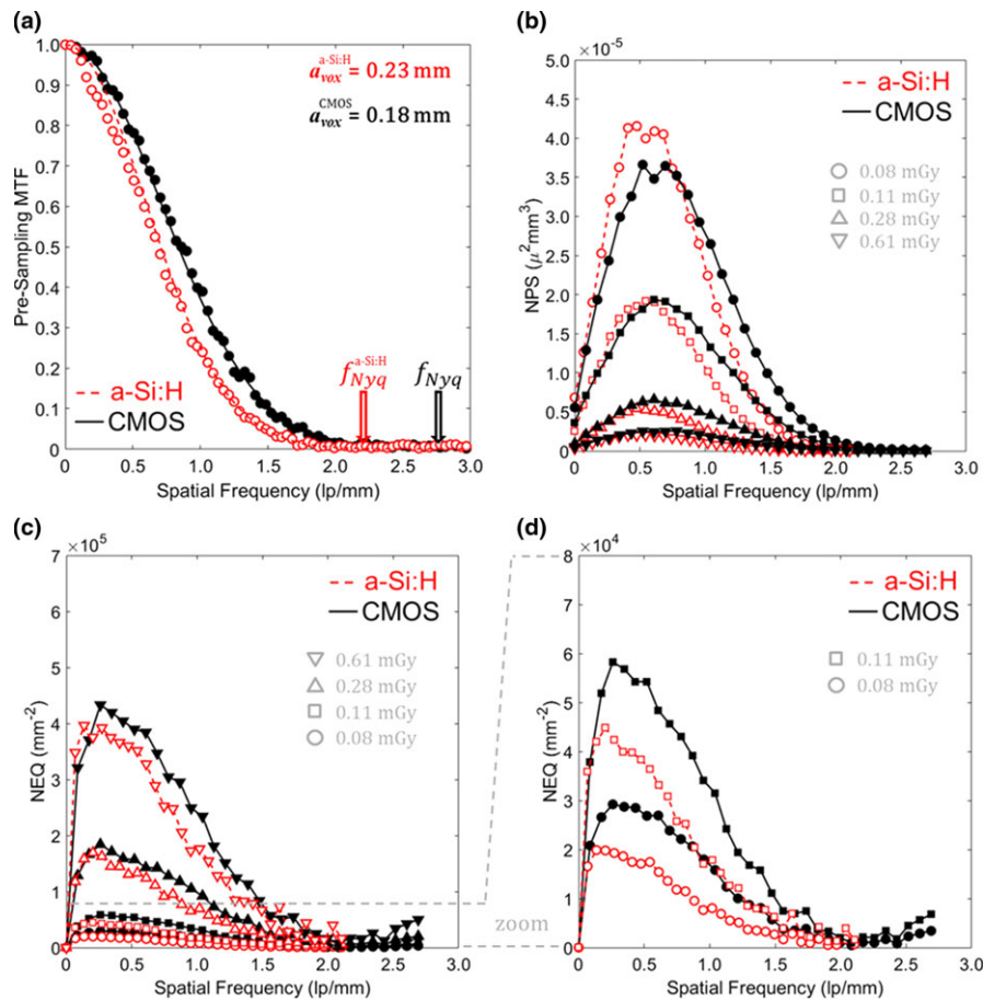
FIG. 12. 3D MTF, NPS, and NEQ for each system with the “Sharp” 3D reconstruction protocol: (a) MTF, (b) NPS, (c) NEQ, and (d) zoom-in of NEQ at lowest dose levels. [Color figure can be viewed at wileyonlinelibrary.com ]
