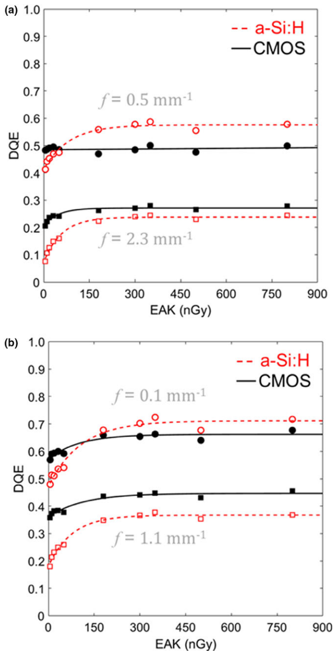
FIG. 7. DQE at low and high-frequency measured as a function of EAK for each system in HG mode with (a) 1 \times 1 and (b) 2 \times 2 binning. Numerous tradeoffs are evident, including the impact of electronic noise at low doses (higher DQE for CMOS) and the impact of reduced optical coupling at higher dose (higher DQE for a-Si:H). [Color figure can be viewed at wileyonlinelibrary.com ]
