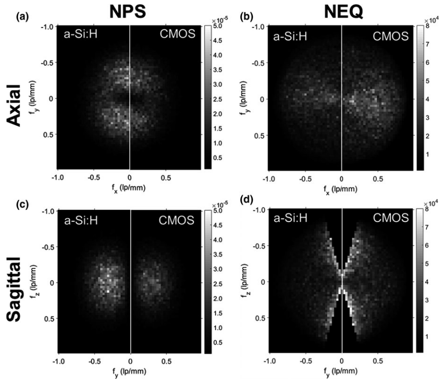
FIG. 10. 3D NPS and NEQ for the “Smooth” reconstruction protocol. Illustrations taken at lowest dose level (0.08 mGy CTDI w ) for: (a) Central axial NPS, (b) Central axial NEQ, (c) Central sagittal NPS and (d) Central sagittal NEQ
