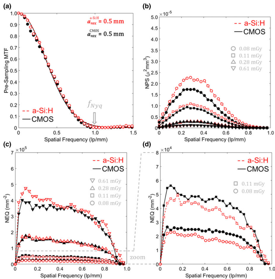
FIG. 9. 3D MTF, NPS, and NEQ for each system with the “Smooth” 3D reconstruction protocol. (a) MTF, (b) NPS, (c) NEQ, and (d) zoom-in of NEQ at the lowest dose levels. [Color figure can be viewed at wileyonlinelibrary.com]
