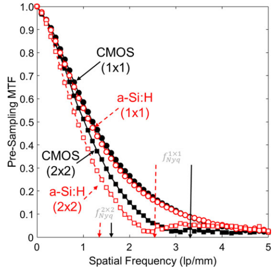
FIG. 4. Pre-sampling MTF in 2D projections for the 1 \times 1 and 2 \times 2 binning modes of each detector. [Color figure can be viewed at wileyonlinelibrary.com]
