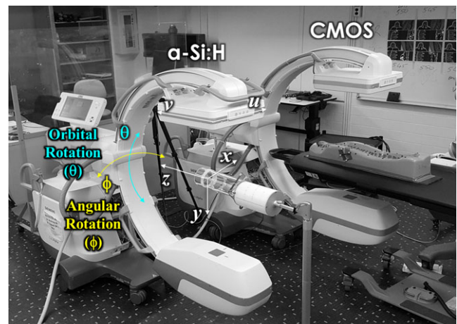
FIG. 1. Experimental setup. Mobile C-arms for 2D and 3D imaging. The systems were identical except for the detector type – that is, a-Si:H or CMOS FPDs. [Color figure can be viewed at wileyonlinelibrary.com]
