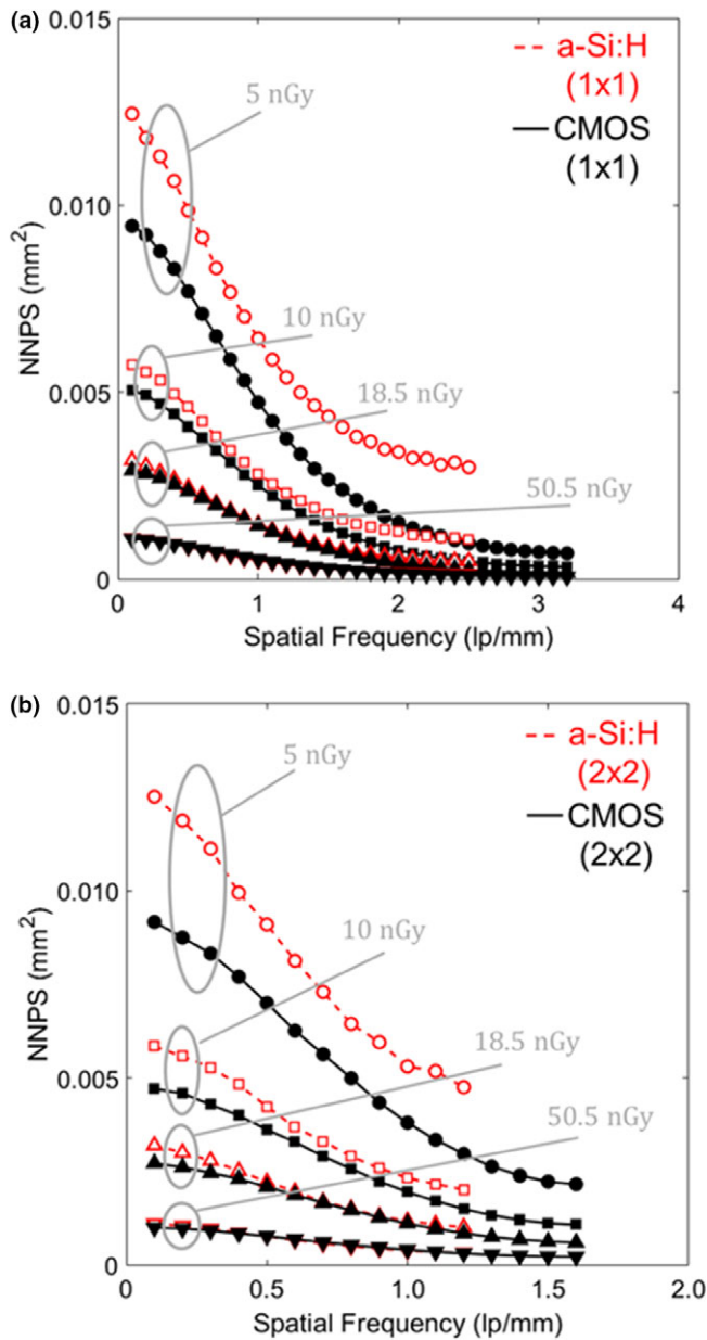
FIG. 5. Projection image NNPS in HG for the (a) 1 \times 1 and (b) 2 \times 2 binning modes at low-dose levels for which electronic noise contributes substantially to the total noise. [Color figure can be viewed at wileyonlinelibrary.com]
