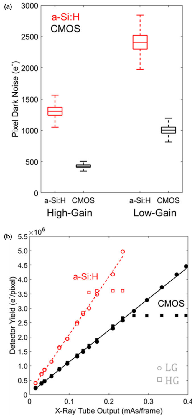
FIG. 2. (a) Pixel dark noise for CMOS and a-Si:H detector in HG and LG modes. (b) Gain and linearity of detector response. [Color figure can be viewed at wileyonlinelibrary.com ]
