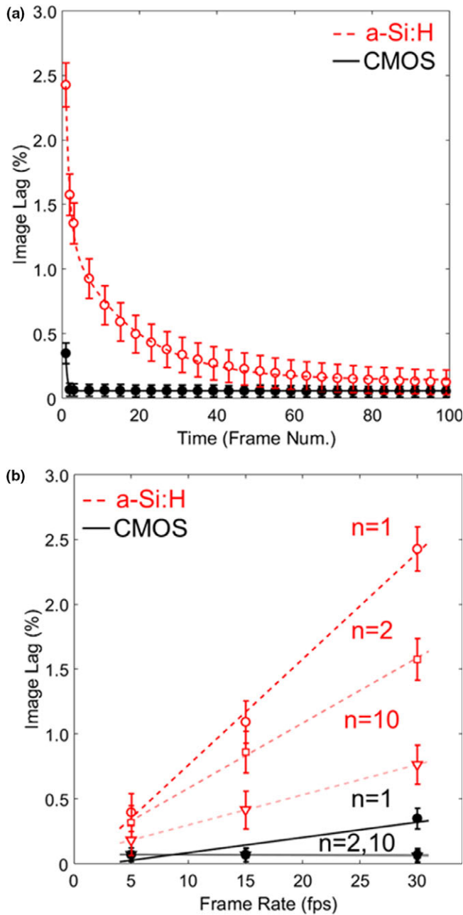
FIG. 3. Image lag. (a) Falling-edge response for CMOS and a-Si:H detectors at 30 fps. (b) The n th-frame image lag for each detector at various frame rates. [Color figure can be viewed at wileyonlinelibrary.com]
