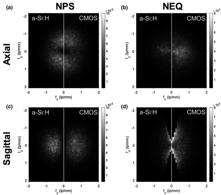
FIG. 13. 3D NPS and NEQ for the “Sharp” reconstruction protocol at low-dose ( CTDI_w = 0.08 mGy). (a) Central axial NPS. (b) Central axial NEQ. (c) Central sagittal NPS. (d) Central sagittal NEQ.
