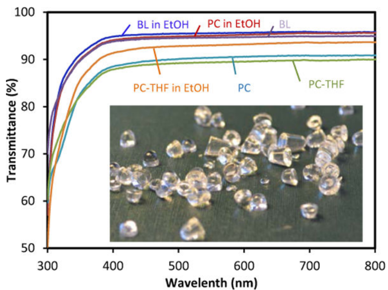
Fig. 4. Optical (transmittance) properties of the BPA-free PCs prepared from DTMPC (0.33 mmol) with 1.7 \mu\text{mol} DBU and 35 \mu\text{mol} 13PDO at 130°C for 1hr. BL in EtOH; Blank in ethanol, PC in EtOH; PC in ethanol, BL; blank, PC-THF in EtOH; PC (after submerged in THF for 15 min) in ethanol, PC; PC, PC-THF; PC after submerged in THF for 15 min. Insert shows PC pellets prepared.
