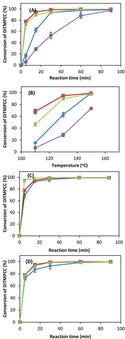
Fig. 1. Synthesis of BPA-free PC from DTMPC (100 mg, 0.33 mmol) by ROP under various conditions. Effect of (A) catalyst system at 130°C and (B) temperature at 15 min in presence of 8.2 μmol DMAP and 35 μmol 1,3PDO (◆), 1.7 μmol DBU and 35 μmol 1,3PDO (■), 0.09 μmol TBD and 35 μmol 1,3PDO (▲), and 7.2 μmol TEA and 35 μmol 1,3PDO (●). C) Effect of temperature under condition of 1.7 μmol DBU and 35 μmol 1,3-PDO at 110°C (◆), 130°C (■) and 150°C (▲). D) Effect of catalyst amount with 0.67 μmol DBU and 35
