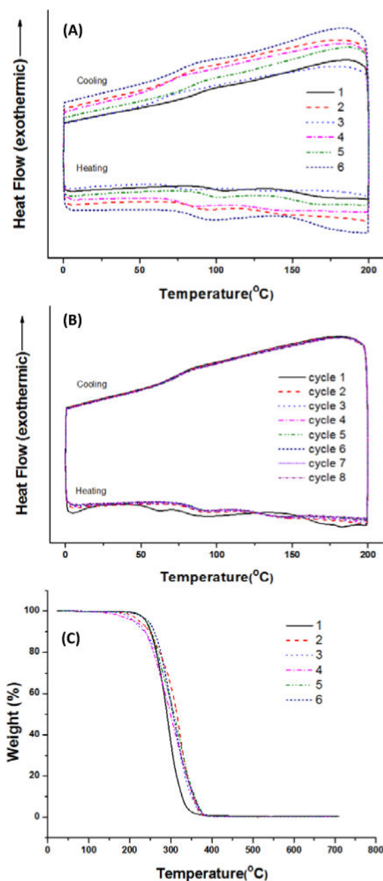
Fig. 5. Thermal properties of the BPA-free PCs prepared from DTMPC (0.33 mmol) by different conditions. (A) DSC graphs for BPA-free PC samples prepared using (1) 1.7 μmol DBU and 3.5 μmol 1,3PDO, (2) 1.7 μmol DBU and 35 μmol 1,3PDO, (3) 1.7 μmol DBU and 70 μmol 1,3PDO, (4) 1.7 μmol DBU and 35 μmol 1,2PDO, (5) 1.7 μmol DBU and 24 μmol 1,6HDO, (6) 1.7 μmol DBU and 140 μmol 1,3PDO at 130°C. (B) DSC cycling graph of BPA-free PC prepared by 1.7 μmol DBU and 35 μmol 1,3-PDO at 130°C. (C) TGA graphs for PC samples prepared by the same condition with (A) DSC samples.
