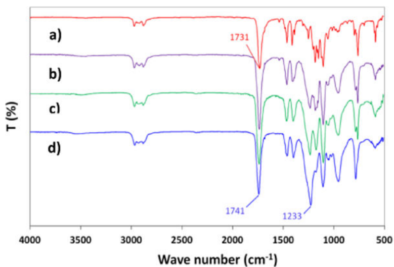
Fig. 3. FT-IR spectra of the reaction components and polycarbonate product formed during ROP of DTMPC at 130 °C. (a) DTMPC, (b) product in 15 min of ROP, (c) product in 30 min in ROP, and (d) product in 120 min in ROP.
