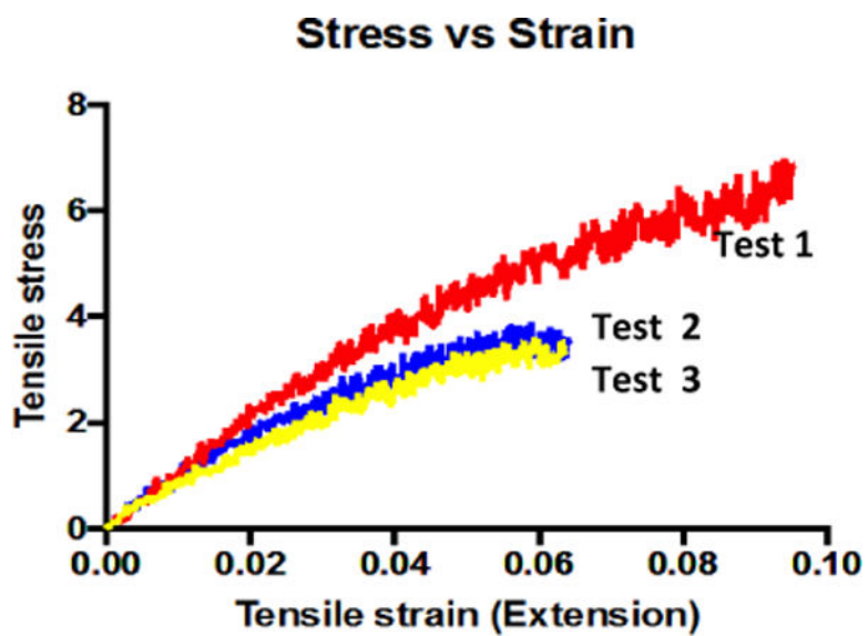
Fig. 6. Tensile mechanical properties of BPA-free PC (PC-T) prepared from 0.33 mmol DTMPC, 0.09 \mu mol TBD and 14 \mu mol 1,3-PDO at 130°C for 1 hr.
