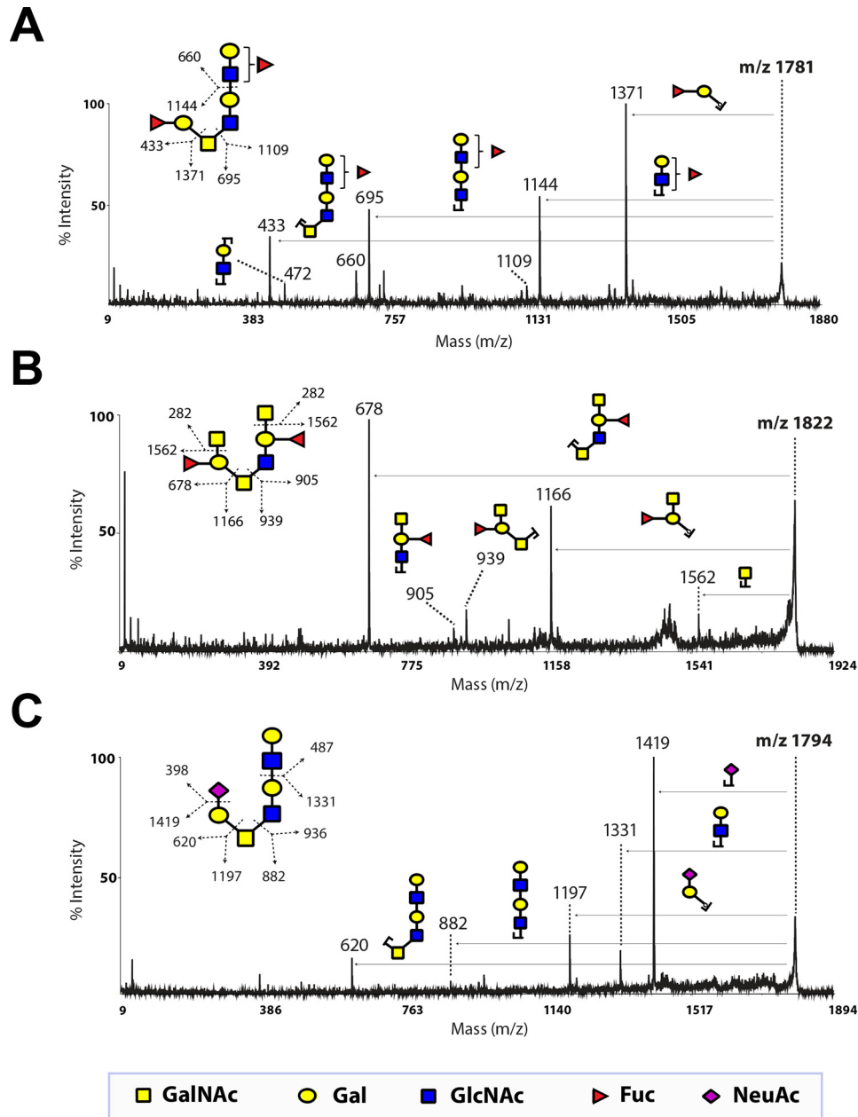
Figure 9. MALDI-TOF/TOF-MS/MS fragmentation spectra confirm the annotation of selected precursor ions from the CEL O-glycome. Molecular ions m/z 1781, 1822, and 1794 from Fig. 8, A–C, respectively, underwent collision-induced dissociation and the resulting fragmentation spectra are shown. Arrows pointing from the dashed line indicate the loss of a specific fragment from the precursor ion. All fragment ions are [M+Na]^+ . When structures have not been unequivocally defined from MS/MS information, the monosaccharide is shown after a bracket.
