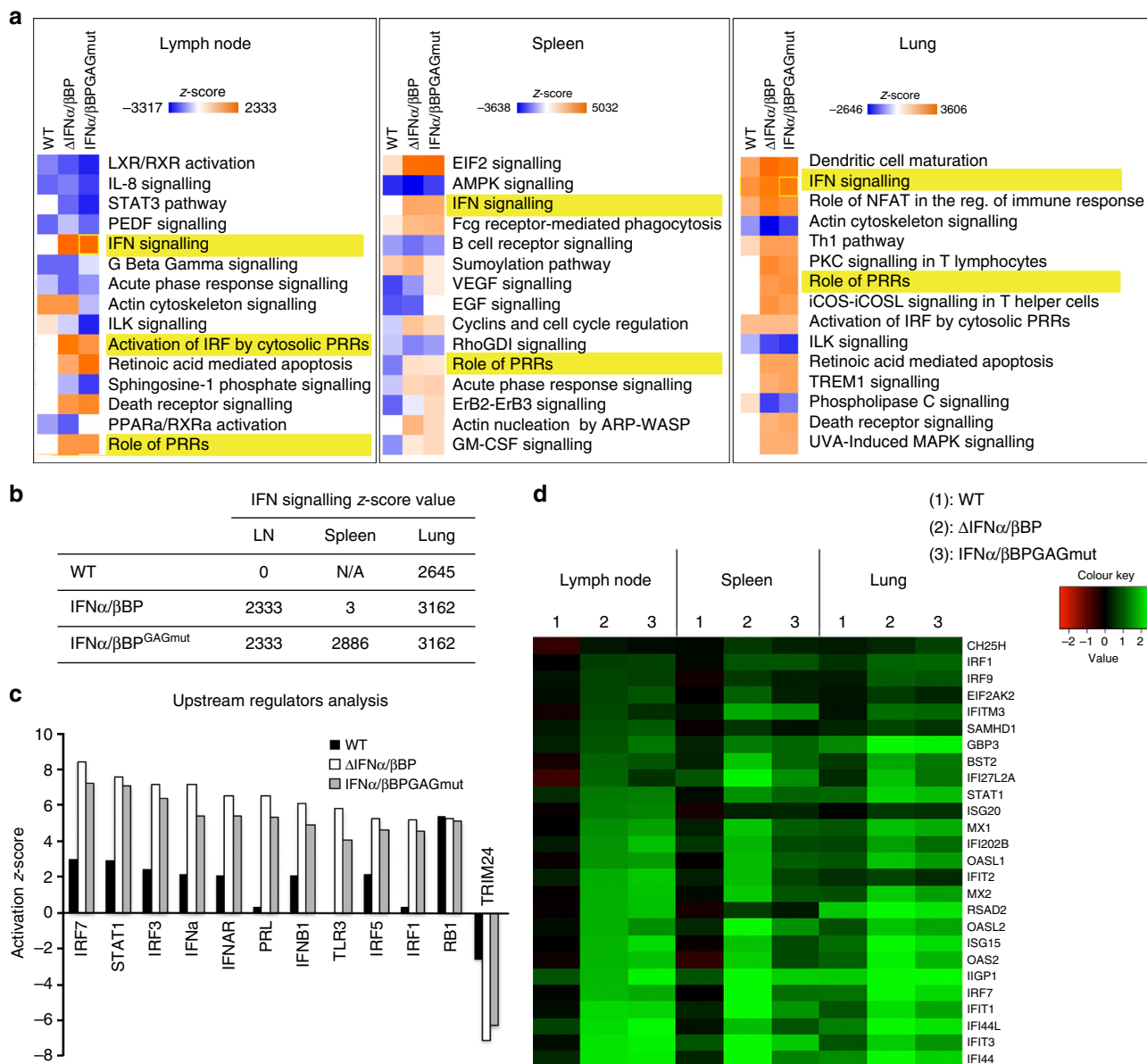
Fig. 9 RNA-seq analysis of the IFN response after infection with VACV IFN \alpha / \beta BP mutants. Two groups of five Balb/c mice per condition were i.n. inoculated with 10^3 pfu of the indicated VACV. Differential expression analyses against mock-infected samples were performed using biological duplicates. a Heatmap showing the activation z-scores for 15 significantly enriched pathways using the SDEGs retrieved after comparison of each VACV infected sample with the mock-infected samples. b Activation z-scores determined for the Interferon Signalling pathway and corresponding to each VACV infected sample after comparison to mock infection. c SDEGs were analysed by the IPA upstream regulator function (direct only) and the activation z-score values for the selected upstream regulators determined for VACV-WT (black bars), VACV \Delta IFN \alpha / \beta BP (white bars) and VACVIFN \alpha / \beta BP GAGmut (grey bars) infections are shown. d Heatmap showing the expression values (log 2 FC) of the selected ISGs in the indicated VACV infected tissues
