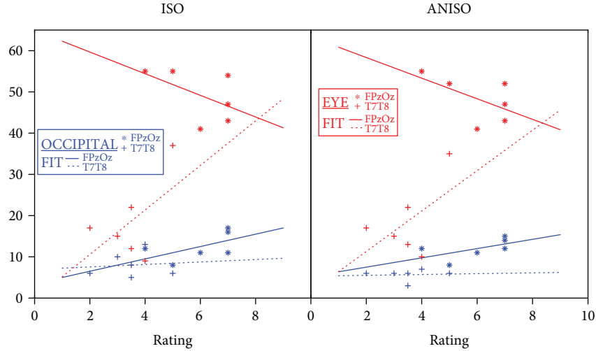
FIGURE 5: Scatter plots comparing subject ratings and median current density percentages (%s) for both Fpz-Oz and T7-T8 montages for (left) isotropic and (right) anisotropic models. Fit lines shown are to median data and illustrate trends only.
