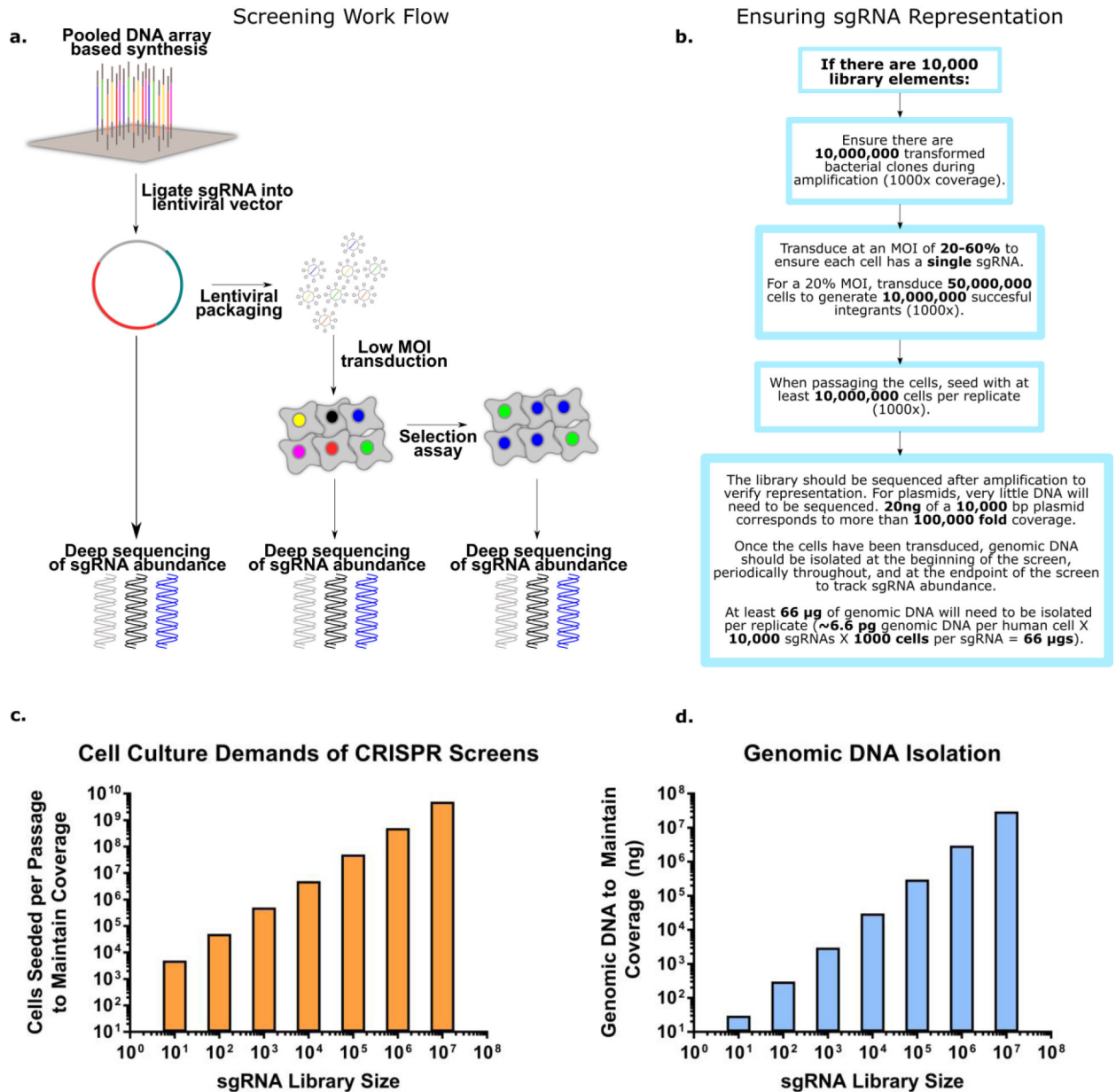
Figure 2. Mechanics of CRISPR-Cas screens:
