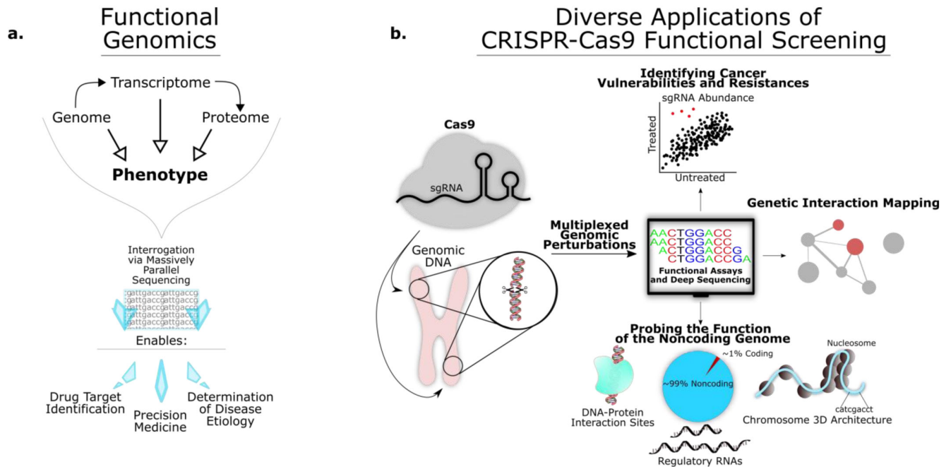
Figure 1. Functional Genomics and CRISPR-Cas:
