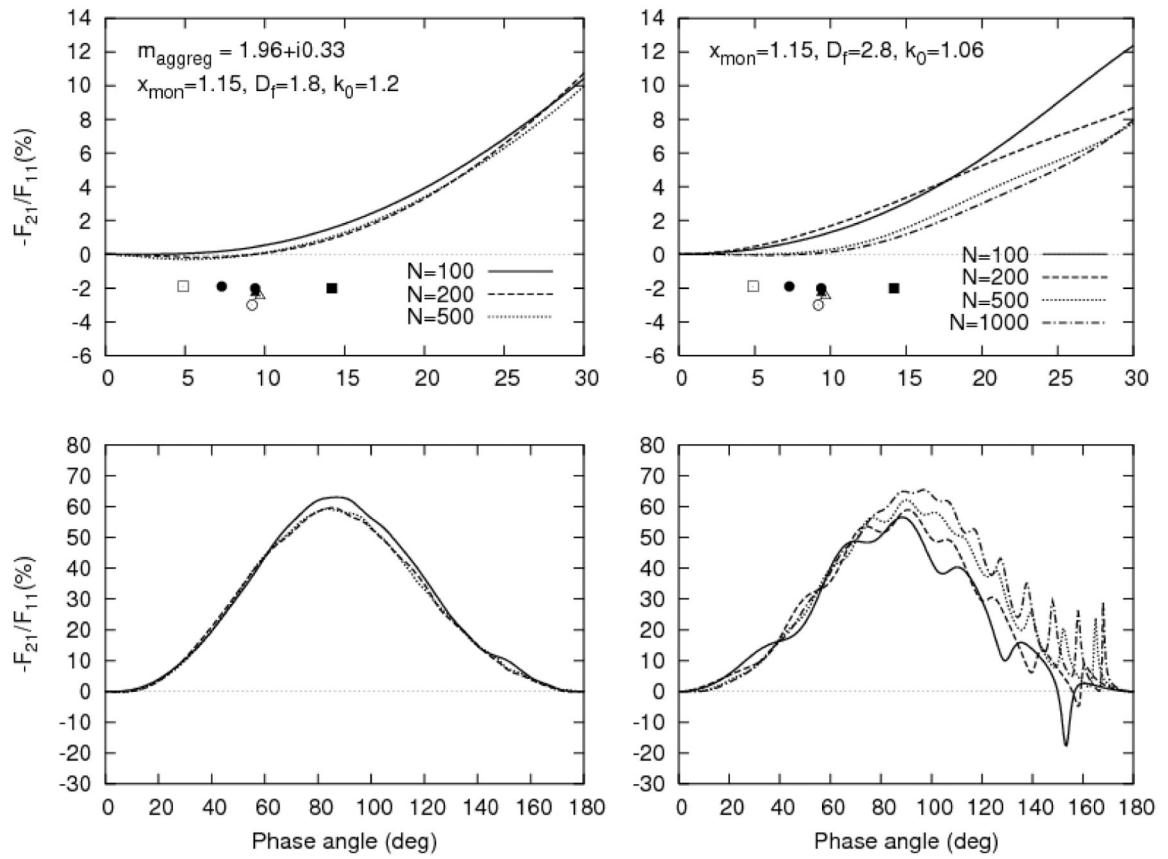
Fig. 8. As in Fig. 5, but for the refractive index m = 1.96 + i0.33 and D_f = 1.8 , k_0 = 1.2 (the left-hand panels) and D_f = 2.8 , k_0 = 1.06 (the right-hand panels).
