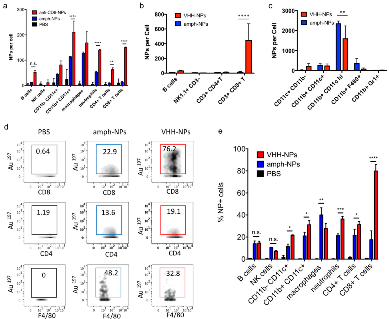
Figure 5. Antibody- and VHH-mediated targeting of nanoparticles to T cells in vivo . (a) C57Bl/6 mice ( n=3 animals/group) were injected i.v. with 150 \mu\text{g} amph-NPs or anti-CD8-NPs, and particle uptake in PBMCs was analyzed 24 hr later by mass cytometry. (b-d) C57Bl/6 mice ( n=3 animals/group) were injected i.v. with 100 \mu\text{g} amph-NPs or VHH-NPs. Twenty-four hr later particle uptake in leukocytes was analyzed by mass cytometry. Shown is uptake in peripheral blood lymphocytes (b) and myeloid cells (c), representative mass cytometry plots from several cell populations showing percentages of NP + cells (d), and quantitation of the mean NP + cells (e). **** p < 0.0001 ; ***, p < 0.001 ; **, p < 0.01 ; *, p < 0.05 ; n.s. not significant by two-way ANOVA with Tukey's multiple comparison test.
