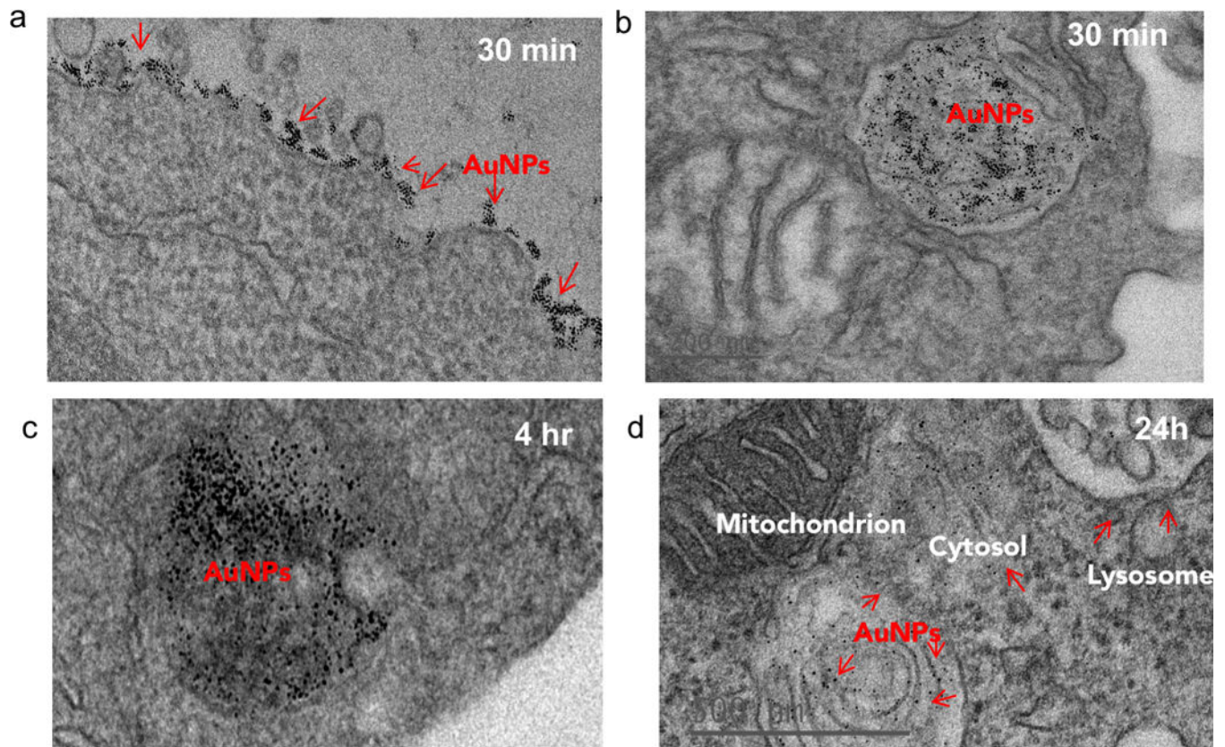
Figure 4. TEM imaging of antibody-targeted amph-NP uptake by CD8 + T cells.
