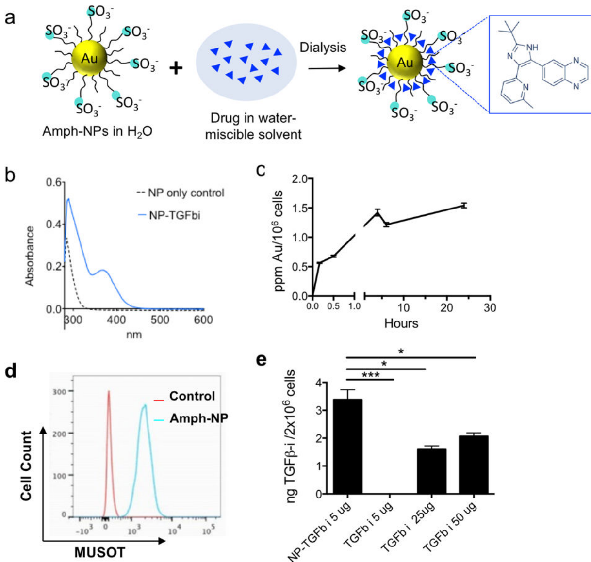
Figure 1. TGF-βi drug loading, quantification and cellular uptake in CD8 + T cells in vitro . (a) Schematic illustration of small molecule TGF-βi sequestration in the amphiphilic ligand shell of amph-NPs. (b) Unloaded amph-NPs or amph-NPs loaded with TGF-βi were treated with β-mercaptoethanol to disrupt the ligand shell followed by UV-vis absorbance measurements to detect released TGF-βi. (c) Primary CD8 + T cells from C57Bl/6 mice were incubated with 0.1 mg/mL amph-NPs at 37°C for varying times and then total gold content was assessed by ICP-OES ( n =3 samples/condition). (d) CD8 + T cells were incubated with 0.1 mg/mL BODIPY-labeled amph-NPs at 37°C for 3 hr and then analyzed by flow cytometry, compared to unmanipulated control T cells. (e) Primary murine CD8 + T cells were incubated in serum-containing medium with NP-TGF-βi or free TGF-βi at the indicated drug concentrations for 4 hr, followed by HPLC analysis of intracellular TGF-βi concentrations. *, p < 0.05; *** p < 0.001 by ANOVA with Tukey’s post test.
