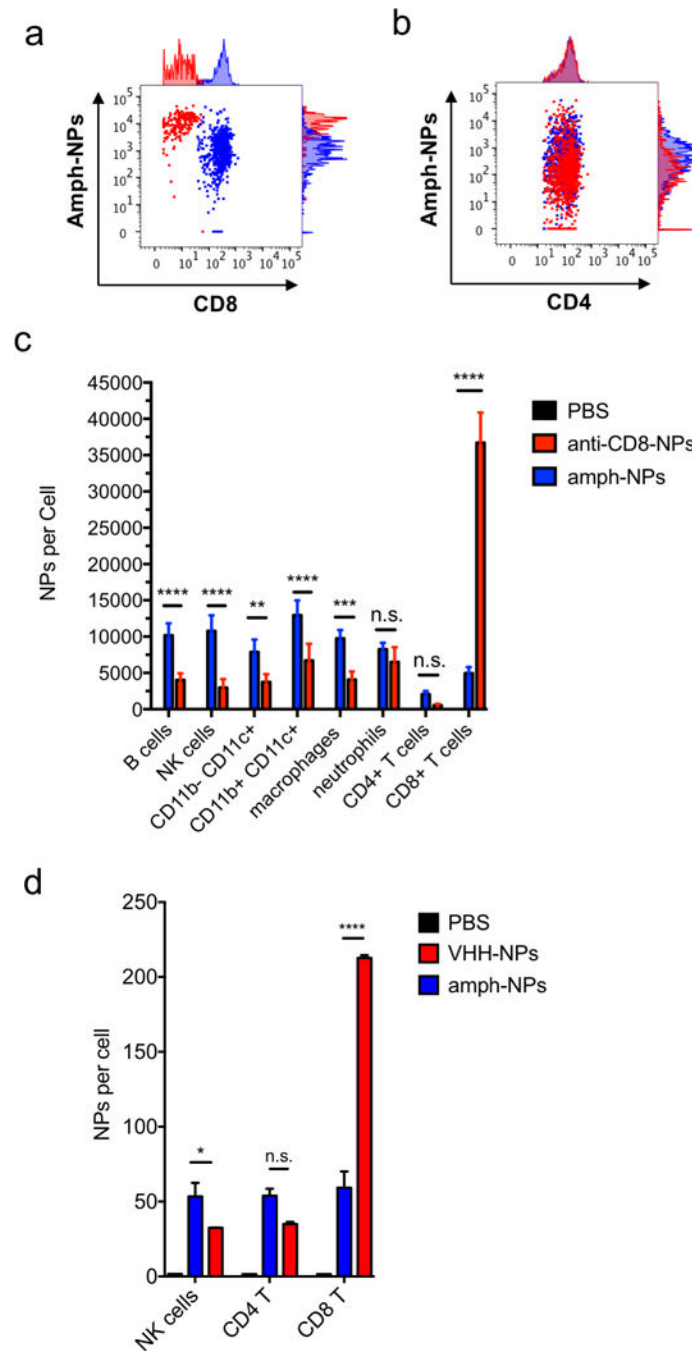
Figure 3. Quantification of antibody-mediated uptake of amph-NPs in lymphocytes in vitro . (a-c) Splenocytes from C57Bl/6 mice were incubated with 10 \mu\text{g}/\text{mL} (gold mass) amph-NPs or anti-CD8-conjugated amph-NPs for 1 hr, then stained with phenotypic antibodies and analyzed by mass cytometry. Shown are representative cytometry graphs overlaying uptake of amph-NPs (blue) and anti-CD8-NPs (red) in CD8 + (a) and CD4 + (b) T cells, and quantitative mean nanoparticle uptake per cell from CyTOF (c, n=3 samples/condition). (d) Splenocytes were incubated with 0.1 \mu\text{g}/\text{mL} amph-NPs or VHH-NPs at 37 ^{\circ}\text{C} for 1 hr then
