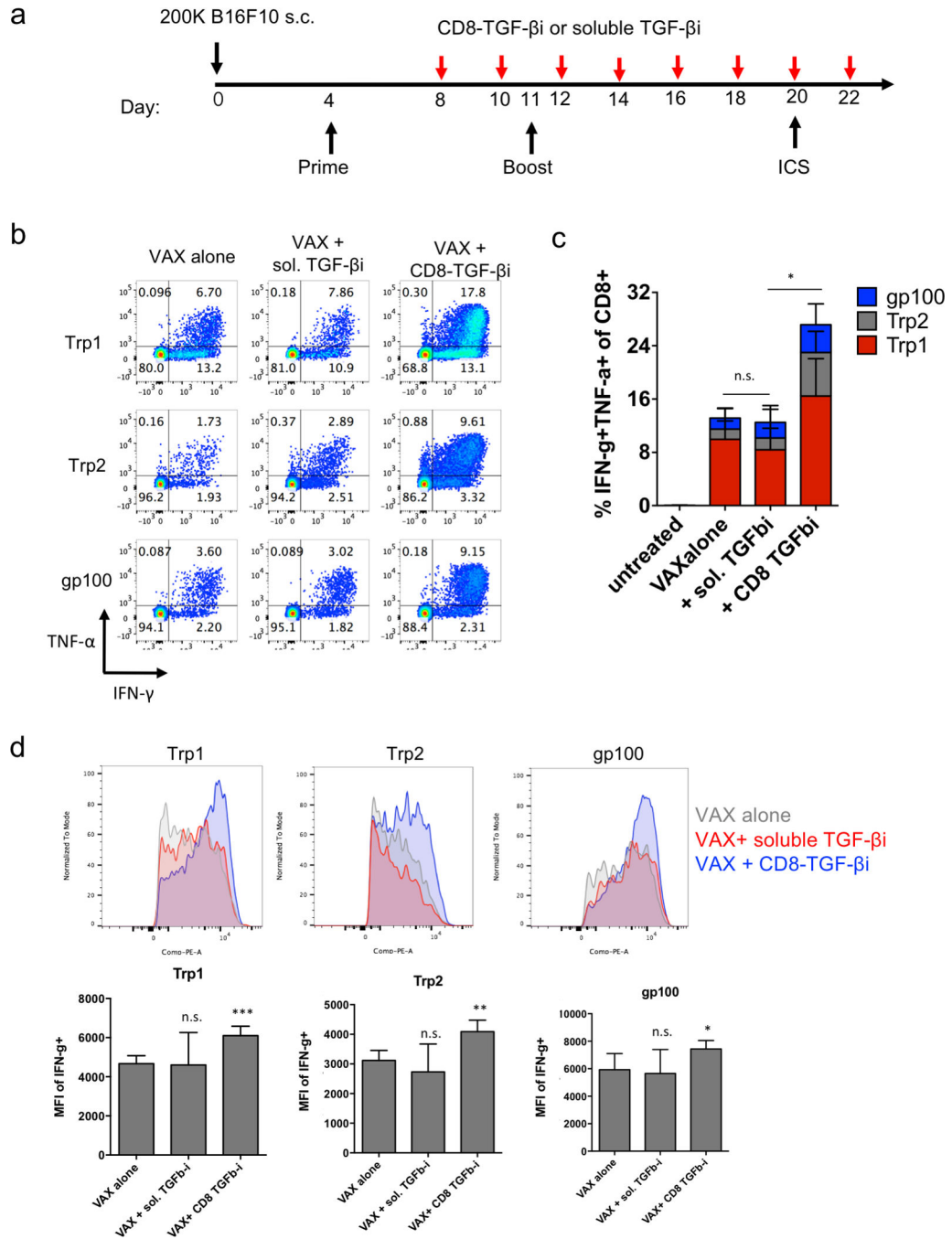
Figure 6. TGFβi delivered via VHH-conjugated amph-NPs augments endogenous CD8 + T cell vaccine responses.
