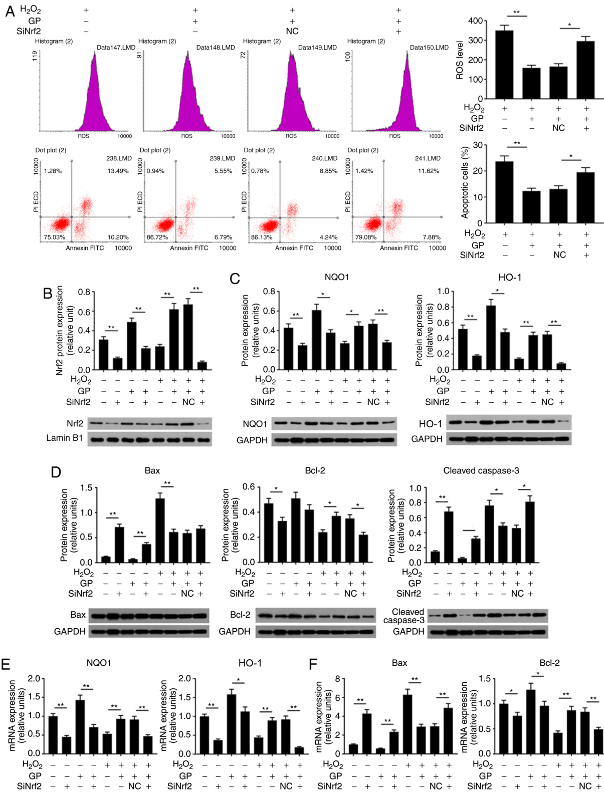
Figure 5. Nrf2 silencing attenuates the effects of GP on H 2 O 2 -induced ARPE-19 cells. (A) ARPE-19 cells were subjected to treatment with 200 μM H 2 O 2 , 30 μM GP, NC vector and siNrf2 vector. Flow cytometry was applied to analyze the levels of ROS and the number of apoptotic cells. *P<0.05, **P<0.01. (B-D) Proteins expression levels of Nrf2, HO-1, NQO1, Bax, Bcl-2 and cleaved-caspase 3 were determined by western blotting. (E and F) mRNA expression levels of HO-1, NQO1, Bax and Bcl-2 were detected by reverse transcription-quantitative polymerase chain reaction. *P<0.05, **P<0.01. n=4. Bcl-2, B-cell lymphoma 2; Bax, Bcl-2-associated X; FITC, fluorescein isothiocyanate; HO-1, heme oxygenase-1; NQO1, NAD(P)H: Quinine oxidoreductase; Nrf2, nuclear factor-erythroid 2-related factor-2; PI, propidium iodide; siNrf2, small interfering RNA Nrf2.
