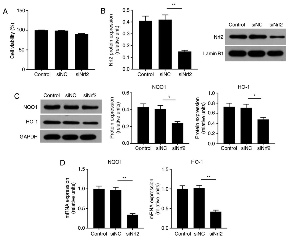
Figure 3. Nrf2 downregulation inhibits the expression of downstream target genes NQO1 and HO-1 in ARPE-19 cells. (A) ARPE-19 cells were transfected with siNC and siNrf2 vectors using Lipofectamine ® 3000. Cell viability was analyzed by an MTT assay. (B and C) Western blotting was applied to detect the expression of Nrf2, HO-1 and NQO1 proteins. (D) Reverse transcription-quantitative polymerase chain reaction was performed to detect the expression of HO-1 and NQO1 mRNA. * P < 0.05 , ** P < 0.01 . n = 4 . HO-1, heme oxygenase-1; NQO1, NAD(P)H: Quinone oxidoreductase; Nrf2, nuclear factor-erythroid 2-related factor-2; siRNA, small interfering RNA; siNC, siRNA negative control; siNrf2, siRNA Nrf2.
