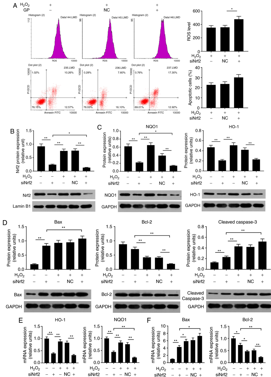
Figure 4. Nrf2 silencing enhances H_2O_2 -induced damage to ARPE-19 cells. (A) ARPE-19 cells were subjected to treatment with 200 \mu M H_2O_2 , NC vector and siNrf2 vector. Flow cytometry was performed to analyze the levels of ROS and the number of apoptotic cells. * P < 0.05 vs. H_2O_2 + NC group. (B) Proteins expression levels of Nrf2, were determined using western blotting. (C) The protein expression levels of NQO1 and HO-1 were detected by reverse transcription-quantitative polymerase chain reaction. (D) The protein expression levels of cleaved-caspase 3, Bax and Bcl-2 were detected by western blotting. (E) The mRNA expression levels of HO-1 and NQO1 were detected by reverse transcription-quantitative polymerase chain reaction. (F) The mRNA expression levels of Bax and Bcl-2 were detected by reverse transcription-quantitative polymerase chain reaction. * P < 0.05 , ** P < 0.01 . n=4. Bcl-2, B-cell lymphoma 2; Bax, Bcl-2-associated X; FITC, fluorescein isothiocyanate; HO-1, heme oxygenase-1; NQO1, NAD(P)H: Quinine oxidoreductase; Nrf2, nuclear factor-erythroid 2-related factor-2; PI, propidium iodide; siRNA, small interfering RNA; NC, siRNA negative control; siNrf2, siRNA Nrf2.
