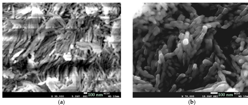
Figure 11. FE-SEM images corresponding to C12GA-templated nanofibrous \text{CePO}_4 annealed at 900\text{ }^\circ\text{C} under \text{N}_2 conditions: (a) Well-preserved nanofibrous region ( \times 35000 ); (b) Higher magnification region ( \times 70000 ) showing thicker, more grown and aggregated nanofibers. Bar length: 100 nm.
