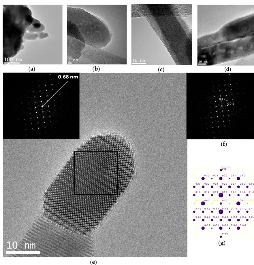
Figure 12. (a–e) HRTEM images of a C12GA-templated \text{CePO}_4 annealed at 900\text{ }^\circ\text{C} under \text{N}_2 conditions, the inset of (e) showing the corresponding digital diffraction pattern (DDP) of the region of the nanofiber marked with an square, with indicated distance; (f) same DDP with some indexed (hkl) values; (g) corresponding simulated kinetic diffraction diagram.
